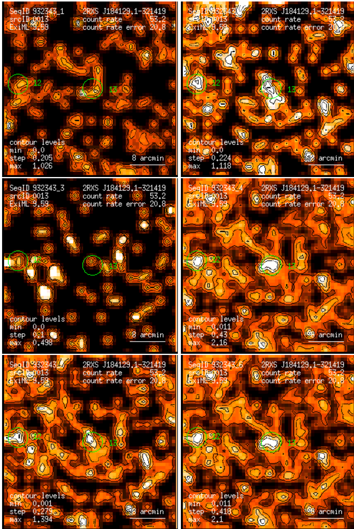
Figure 13: RASS 932343: detection 0013: band rate images, Gaussian filter: (1) PSPC channels 11 – 41, (2) 52 – 90, (3) 91 – 201, (4) 11 – 235, (5) 52 – 201, (6) 11 – 201. Broad band rates in counts/ks. Band rate contour levels in counts/ks/arcmin 2 .
