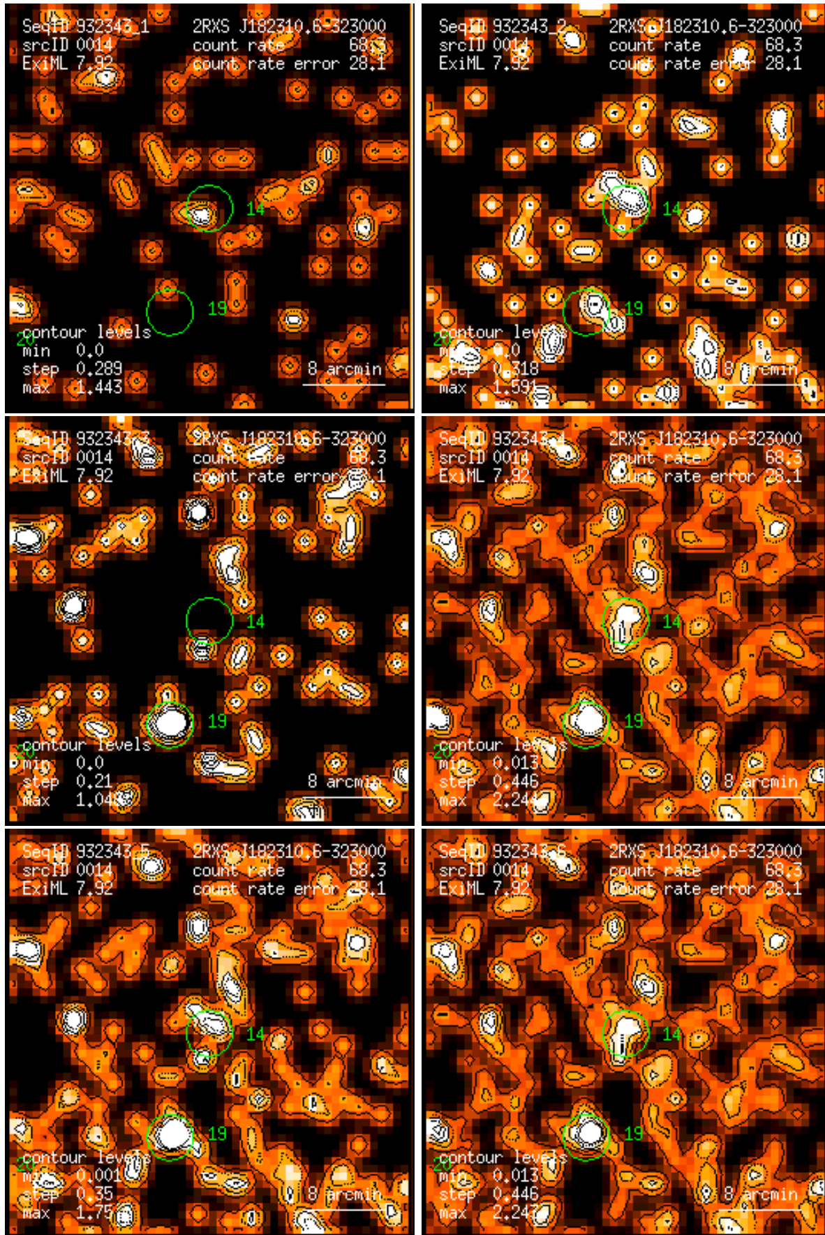
Figure 14: RASS 932343: detection 0014: band rate images, Gaussian filter: (1) PSPC channels 11 – 41, (2) 52 – 90, (3) 91 – 201, (4) 11 – 235, (5) 52 – 201, (6) 11 – 201. Broad band rates in counts/ks. Band rate contour levels in counts/ks/arcmin 2 .
