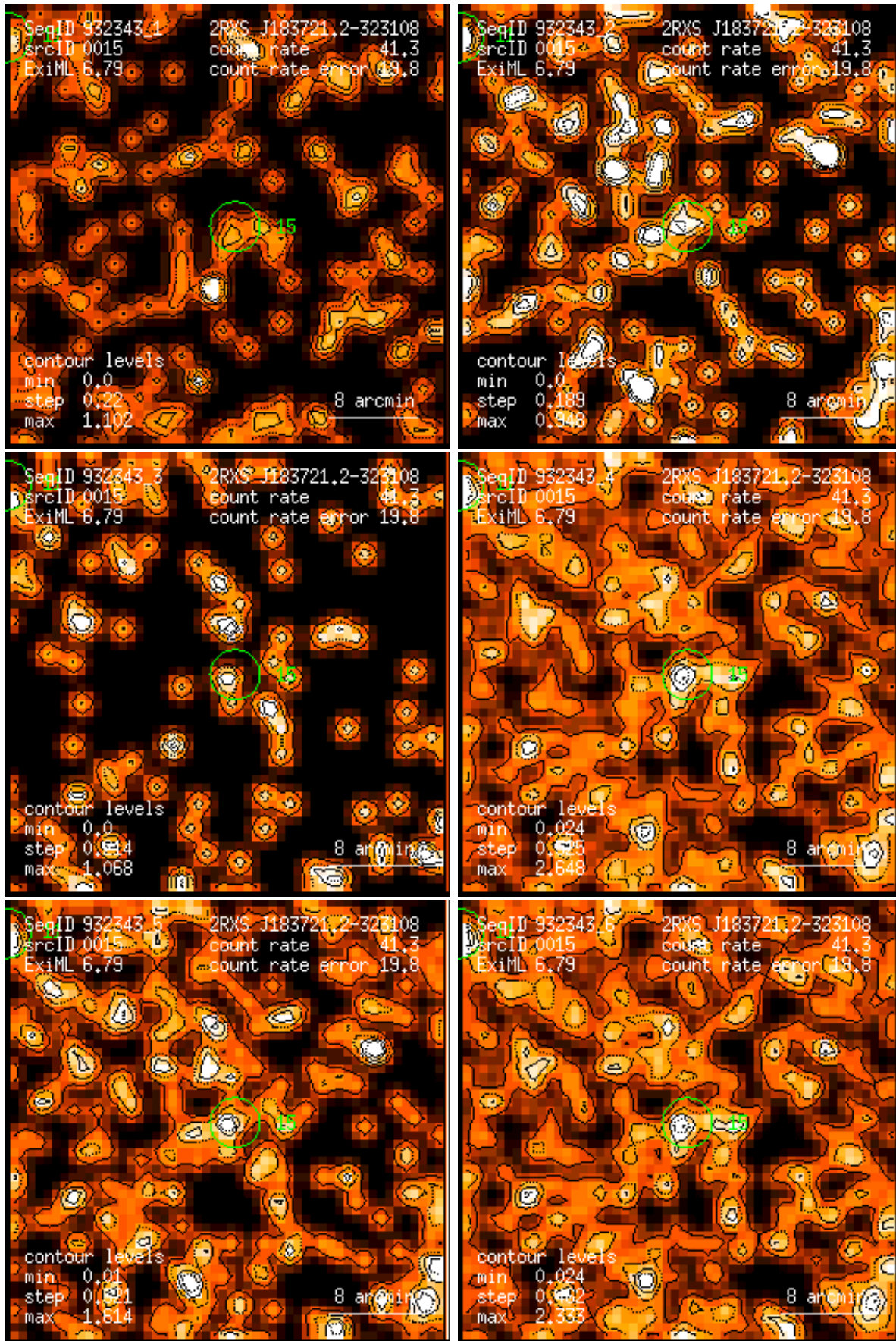
Figure 15: RASS 932343: detection 0015: band rate images, Gaussian filter: (1) PSPC channels 11 – 41, (2) 52 – 90, (3) 91 – 201, (4) 11 – 235, (5) 52 – 201, (6) 11 – 201. Broad band rates in counts/ks. Band rate contour levels in counts/ks/arcmin 2 .
