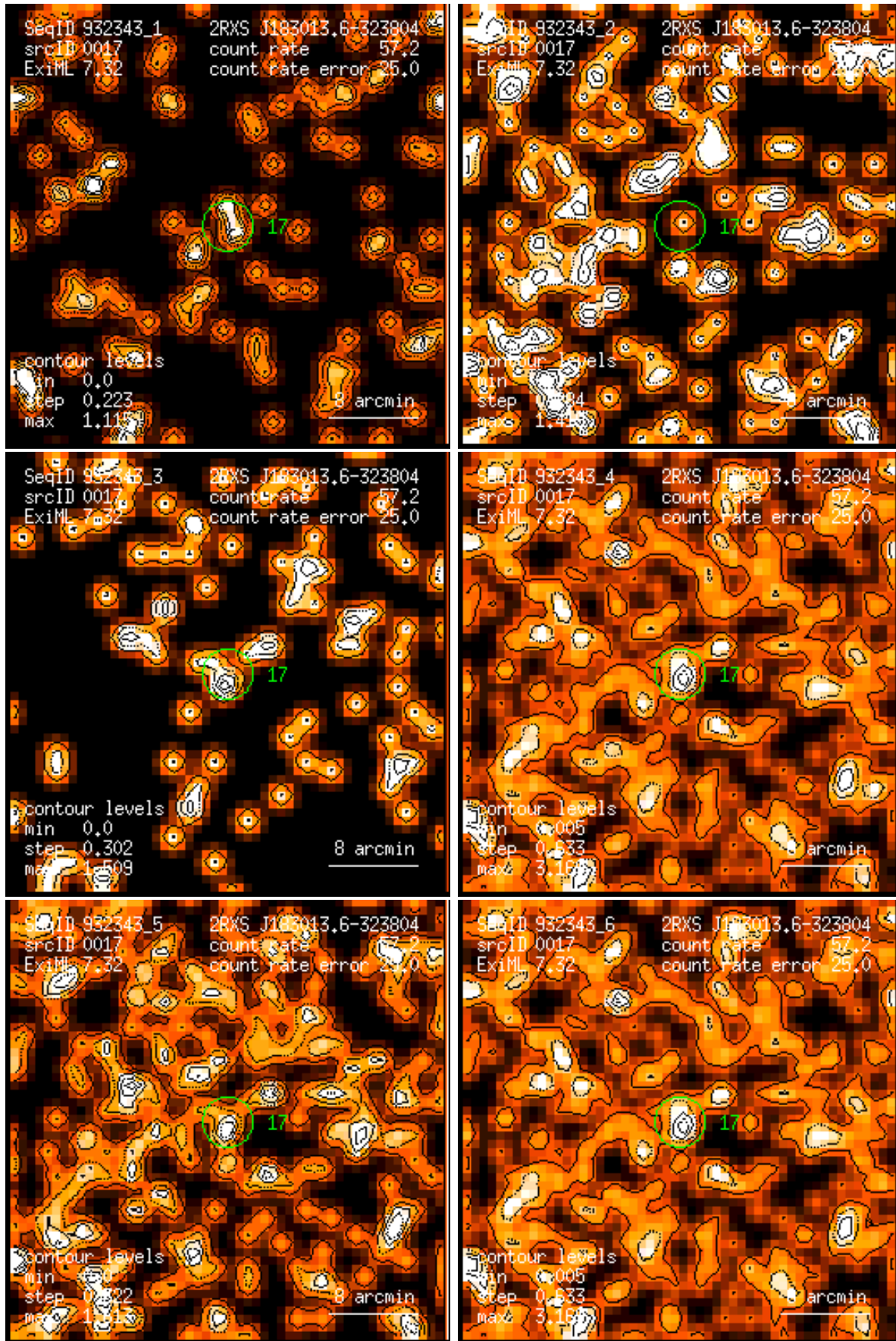
Figure 17: RASS 932343: detection 0017: band rate images, Gaussian filter: (1) PSPC channels 11 – 41, (2) 52 – 90, (3) 91 – 201, (4) 11 – 235, (5) 52 – 201, (6) 11 – 201. Broad band rates in counts/ks. Band rate contour levels in counts/ks/arcmin 2 .
