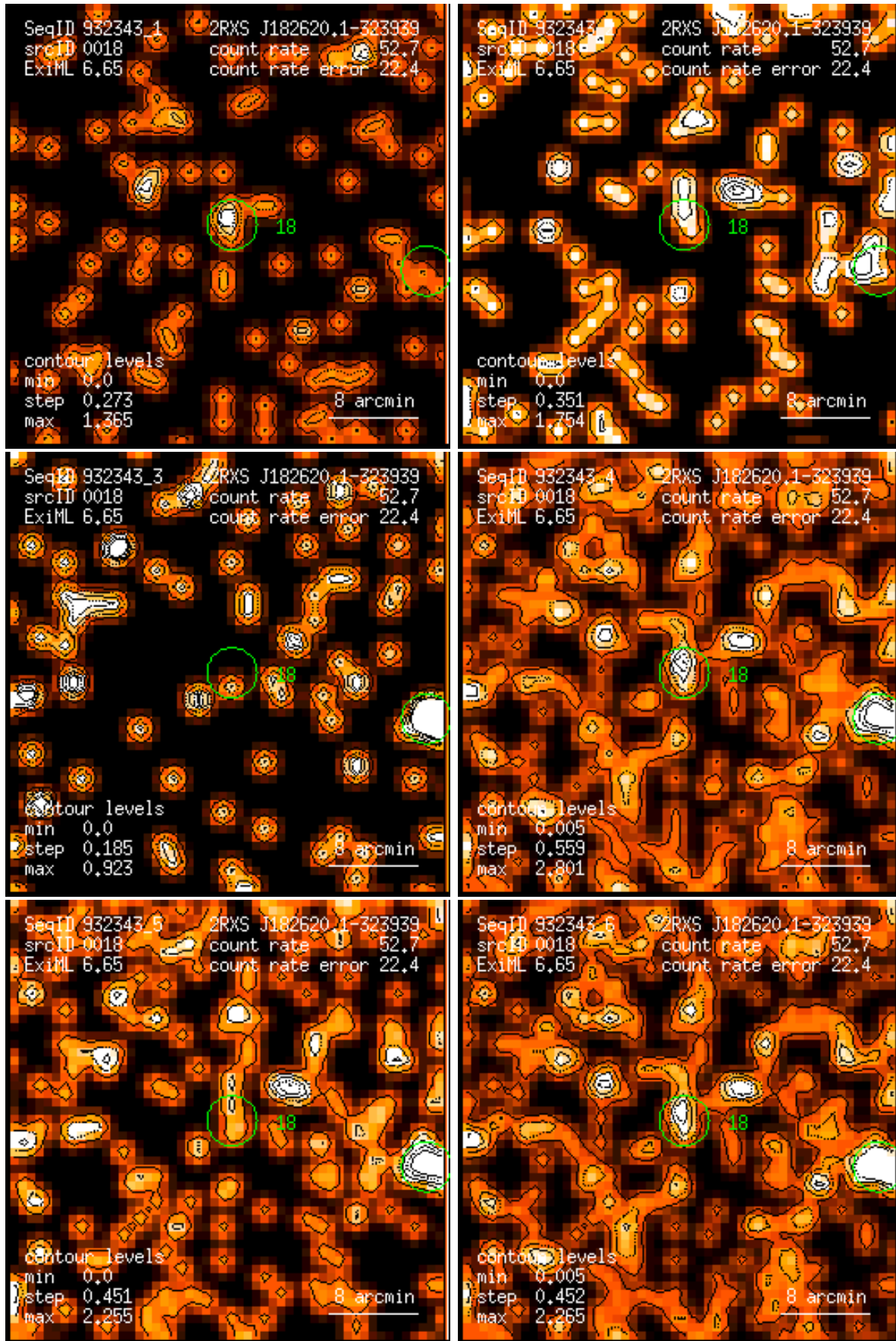
Figure 18: RASS 932343: detection 0018: band rate images, Gaussian filter: (1) PSPC channels 11 – 41, (2) 52 – 90, (3) 91 – 201, (4) 11 – 235, (5) 52 – 201, (6) 11 – 201. Broad band rates in counts/ks. Band rate contour levels in counts/ks/arcmin 2 .
