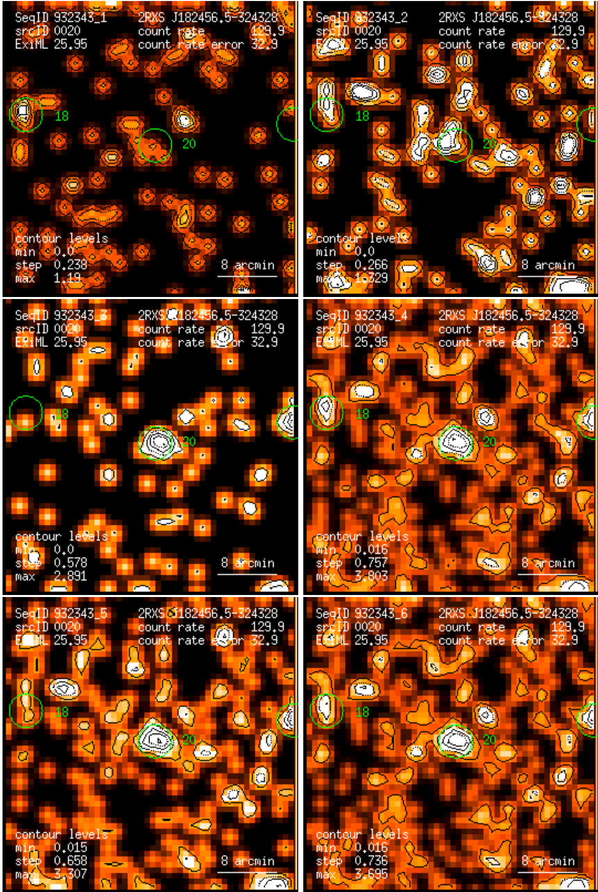
Figure 20: RASS 932343: detection 0020: band rate images, Gaussian filter: (1) PSPC channels 11 – 41, (2) 52 – 90, (3) 91 – 201, (4) 11 – 235, (5) 52 – 201, (6) 11 – 201. Broad band rates in counts/ks. Band rate contour levels in counts/ks/arcmin 2 .
