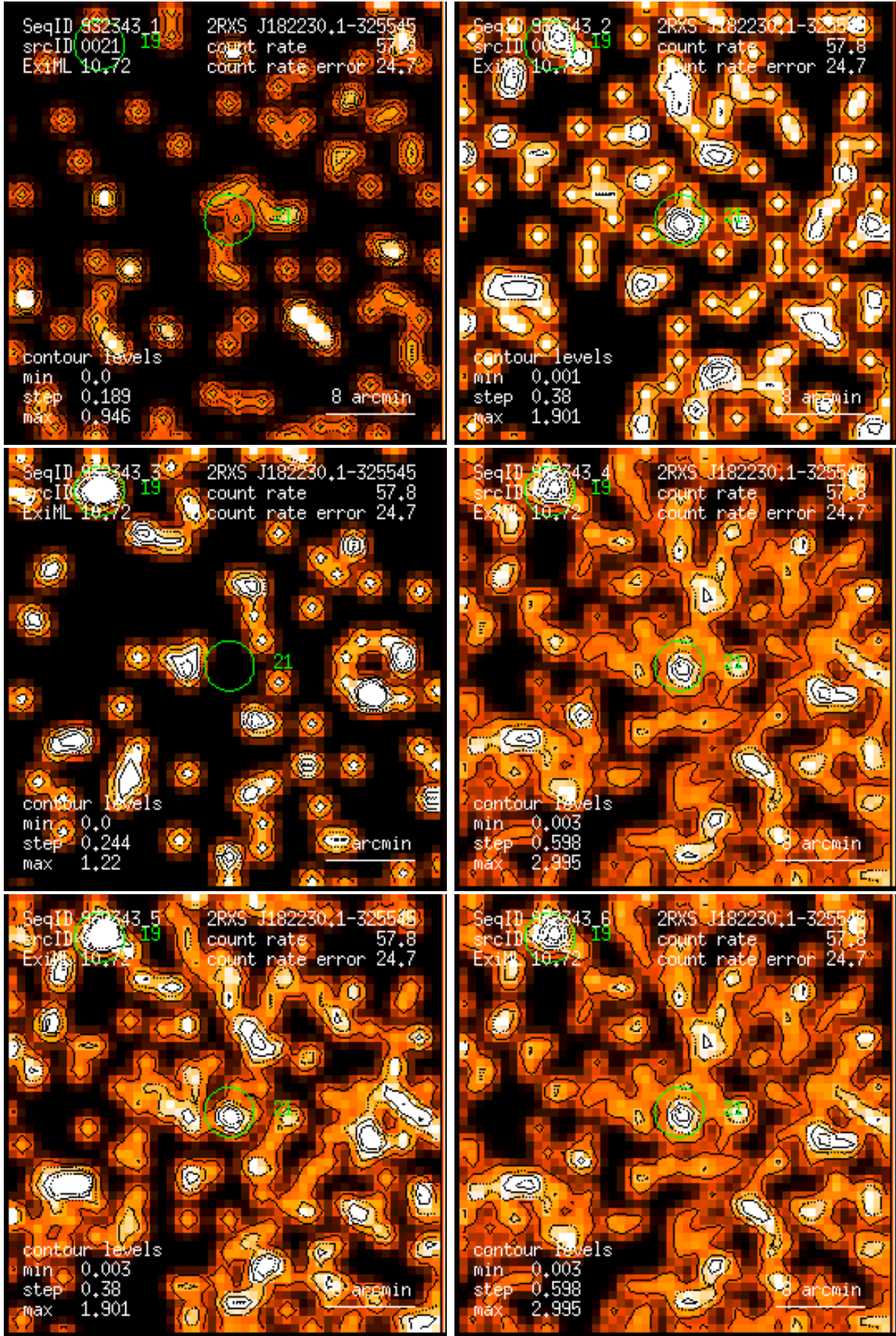
Figure 21: RASS 932343: detection 0021: band rate images, Gaussian filter: (1) PSPC channels 11 – 41, (2) 52 – 90, (3) 91 – 201, (4) 11 – 235, (5) 52 – 201, (6) 11 – 201. Broad band rates in counts/ks. Band rate contour levels in counts/ks/arcmin 2 .
