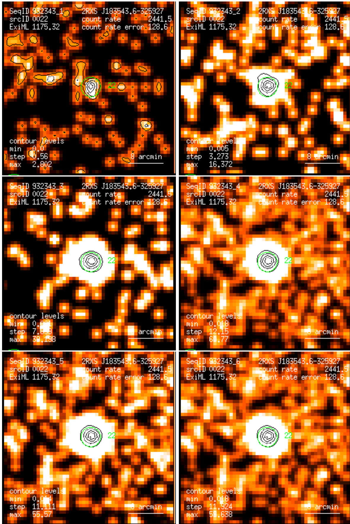
Figure 22: RASS 932343: detection 0022: band rate images, Gaussian filter: (1) PSPC channels 11 – 41, (2) 52 – 90, (3) 91 – 201, (4) 11 – 235, (5) 52 – 201, (6) 11 – 201. Broad band rates in counts/ks. Band rate contour levels in counts/ks/arcmin 2 .
