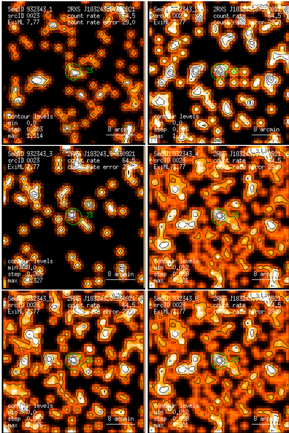
Figure 23: RASS 932343: detection 0023: band rate images, Gaussian filter: (1) PSPC channels 11 – 41, (2) 52 – 90, (3) 91 – 201, (4) 11 – 235, (5) 52 – 201, (6) 11 – 201. Broad band rates in counts/ks. Band rate contour levels in counts/ks/arcmin 2 .
