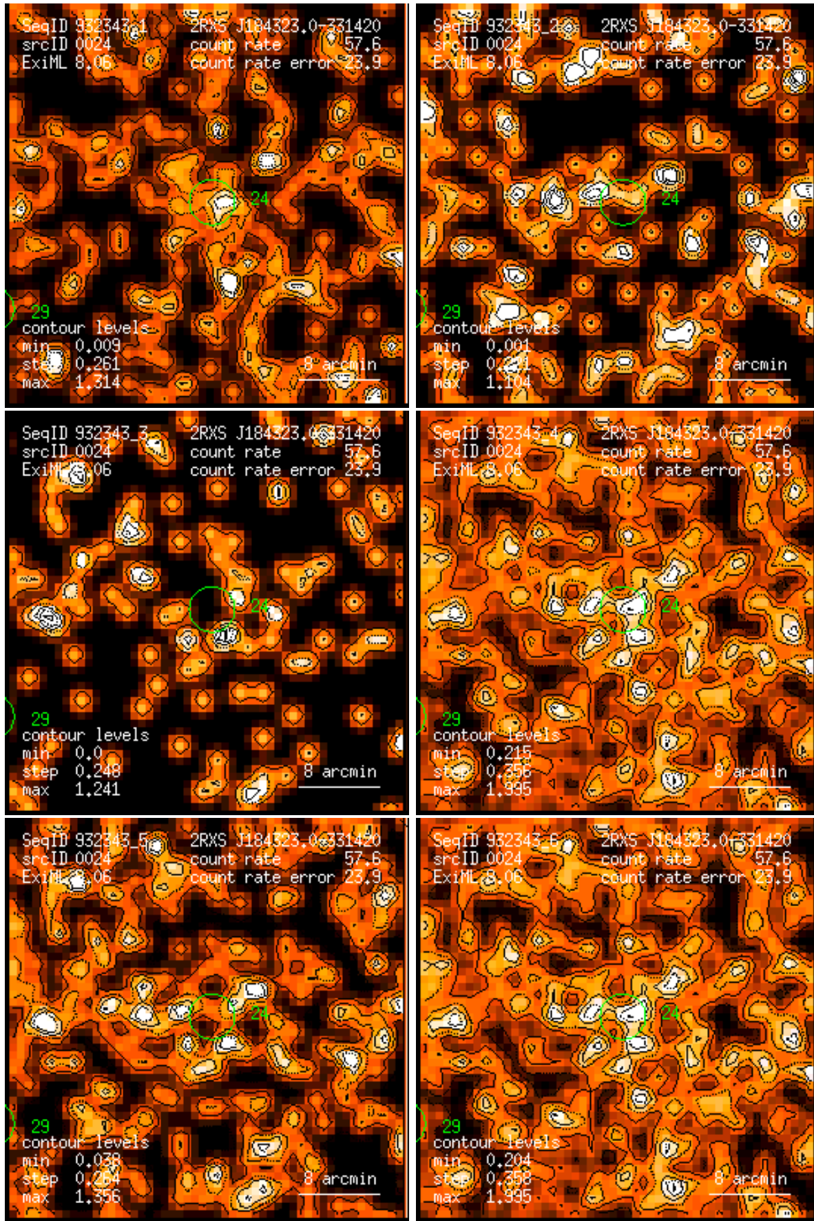
Figure 24: RASS 932343: detection 0024: band rate images, Gaussian filter: (1) PSPC channels 11 – 41, (2) 52 – 90, (3) 91 – 201, (4) 11 – 235, (5) 52 – 201, (6) 11 – 201. Broad band rates in counts/ks. Band rate contour levels in counts/ks/arcmin 2 .
