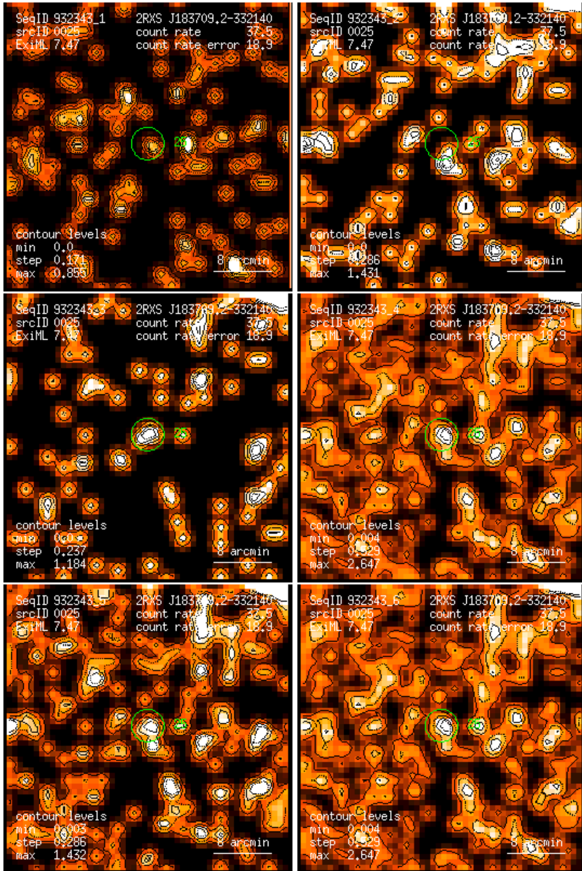
Figure 25: RASS 932343: detection 0025: band rate images, Gaussian filter: (1) PSPC channels 11 – 41, (2) 52 – 90, (3) 91 – 201, (4) 11 – 235, (5) 52 – 201, (6) 11 – 201. Broad band rates in counts/ks. Band rate contour levels in counts/ks/arcmin 2 .
