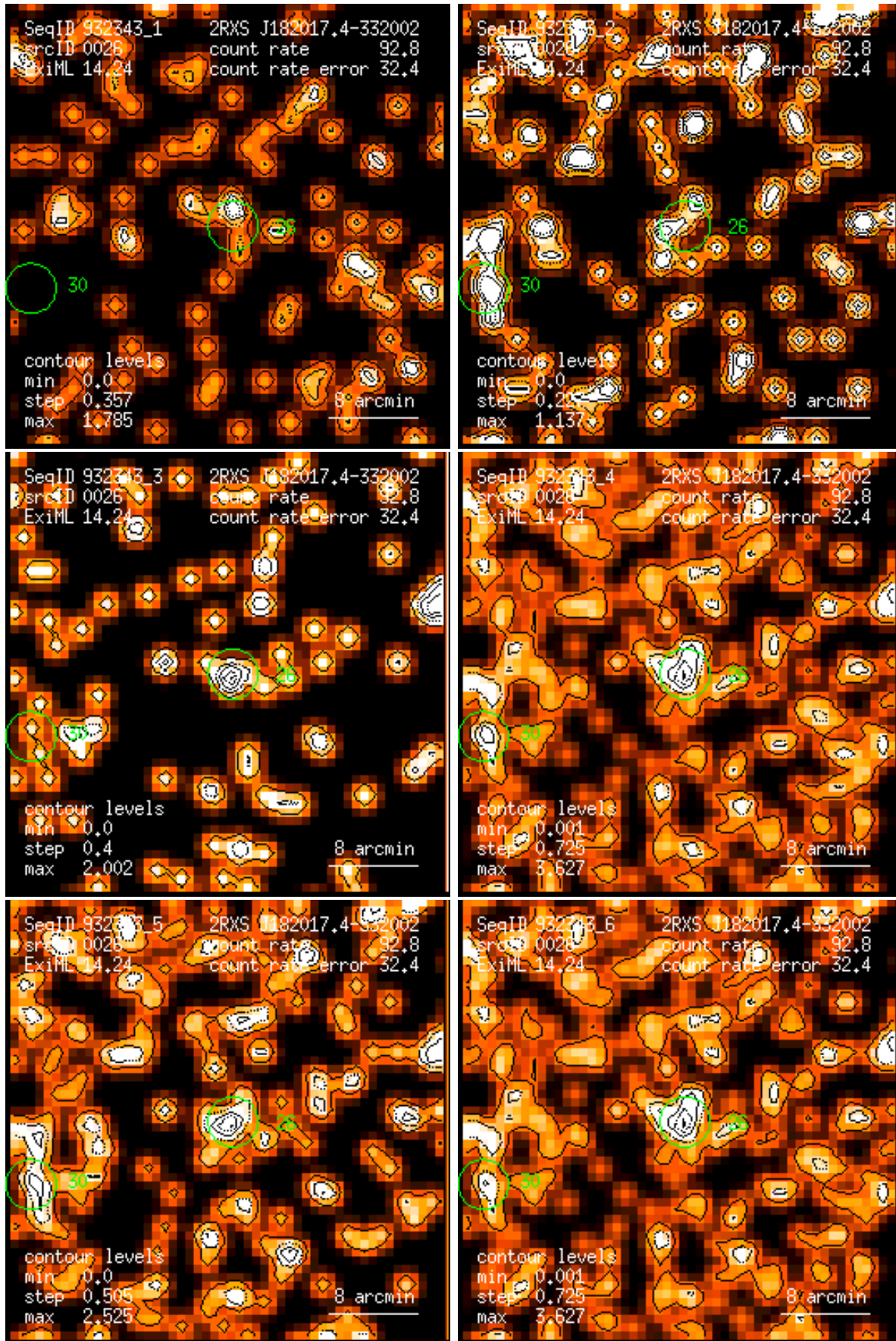
Figure 26: RASS 932343: detection 0026: band rate images, Gaussian filter: (1) PSPC channels 11 – 41, (2) 52 – 90, (3) 91 – 201, (4) 11 – 235, (5) 52 – 201, (6) 11 – 201. Broad band rates in counts/ks. Band rate contour levels in counts/ks/arcmin 2 .
