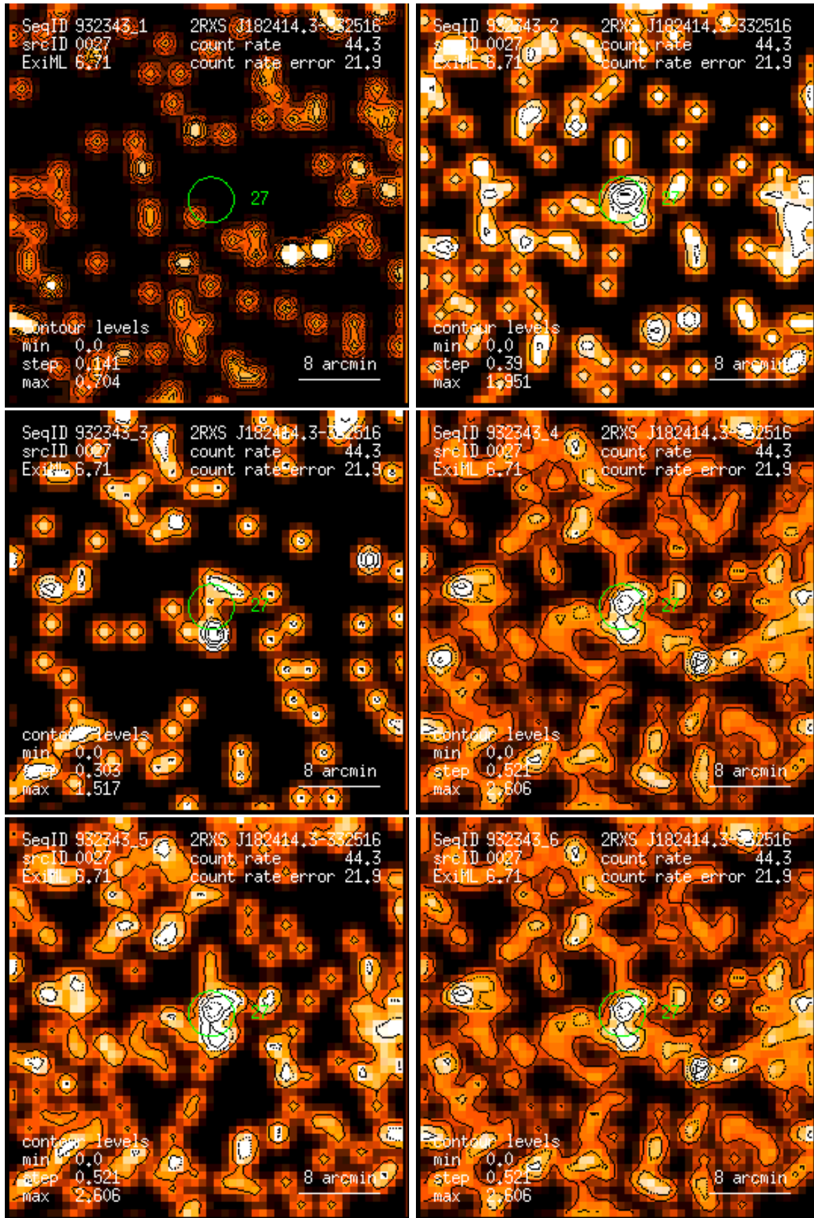
Figure 27: RASS 932343: detection 0027: band rate images, Gaussian filter: (1) PSPC channels 11 – 41, (2) 52 – 90, (3) 91 – 201, (4) 11 – 235, (5) 52 – 201, (6) 11 – 201. Broad band rates in counts/ks. Band rate contour levels in counts/ks/arcmin 2 .
