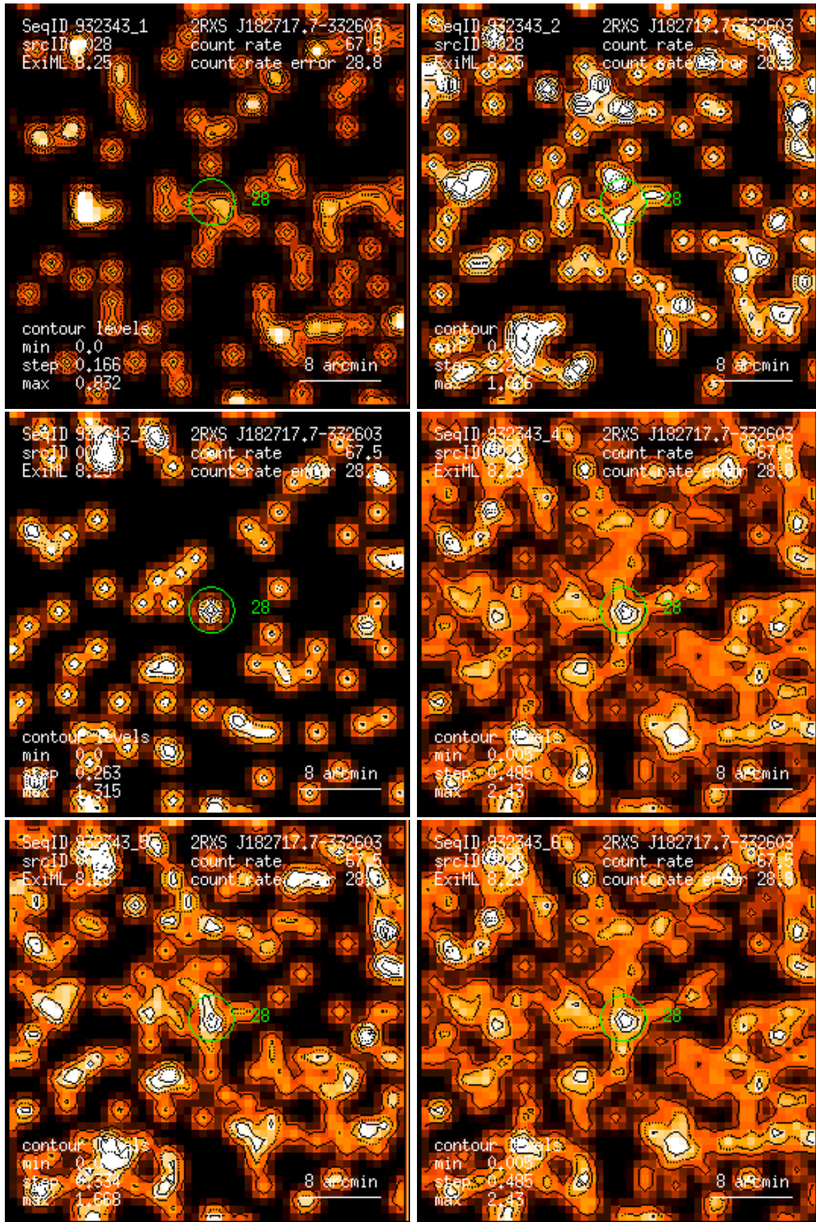
Figure 28: RASS 932343: detection 0028: band rate images, Gaussian filter: (1) PSPC channels 11 – 41, (2) 52 – 90, (3) 91 – 201, (4) 11 – 235, (5) 52 – 201, (6) 11 – 201. Broad band rates in counts/ks. Band rate contour levels in counts/ks/arcmin 2 .
