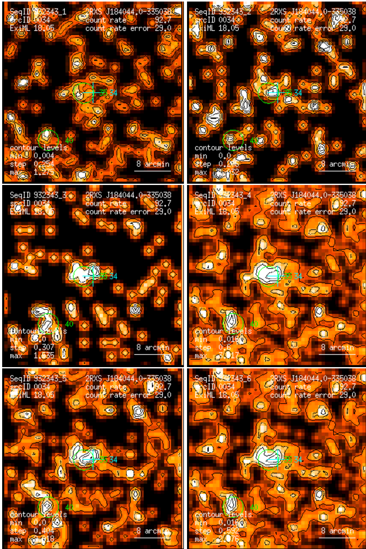
Figure 34: RASS 932343: detection 0034: band rate images, Gaussian filter: (1) PSPC channels 11 – 41, (2) 52 – 90, (3) 91 – 201, (4) 11 – 235, (5) 52 – 201, (6) 11 – 201. Broad band rates in counts/ks. Band rate contour levels in counts/ks/arcmin 2 .
