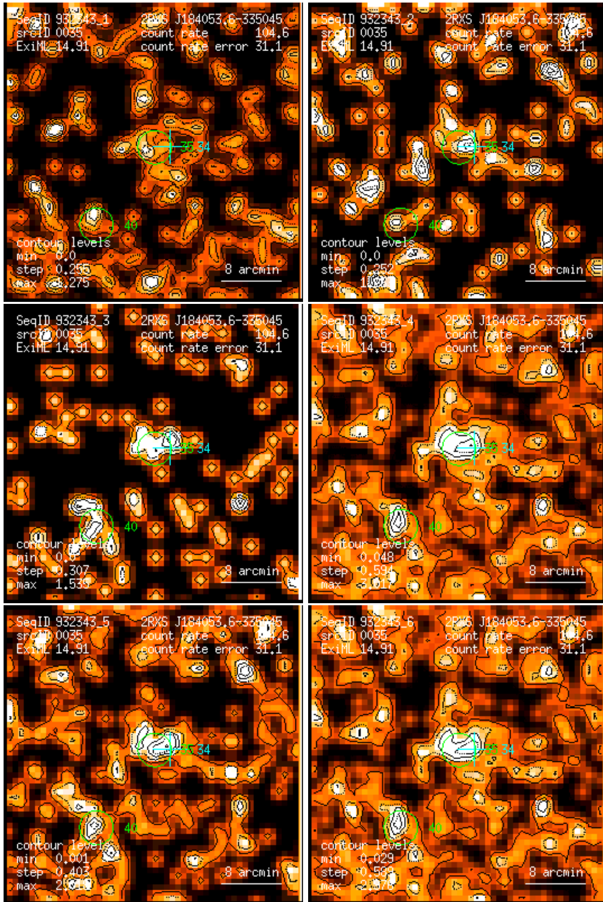
Figure 35: RASS 932343: detection 0035: band rate images, Gaussian filter: (1) PSPC channels 11 – 41, (2) 52 – 90, (3) 91 – 201, (4) 11 – 235, (5) 52 – 201, (6) 11 – 201. Broad band rates in counts/ks. Band rate contour levels in counts/ks/arcmin 2 .
