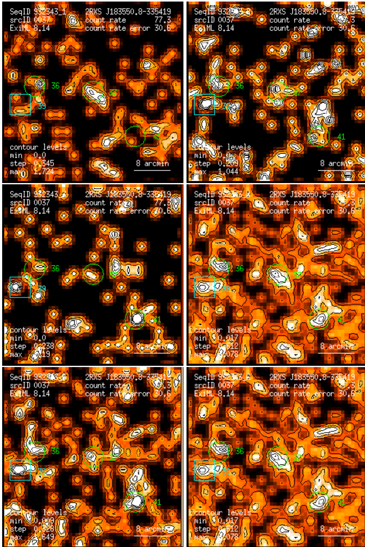
Figure 37: RASS 932343: detection 0037: band rate images, Gaussian filter: (1) PSPC channels 11 – 41, (2) 52 – 90, (3) 91 – 201, (4) 11 – 235, (5) 52 – 201, (6) 11 – 201. Broad band rates in counts/ks. Band rate contour levels in counts/ks/arcmin 2 .
