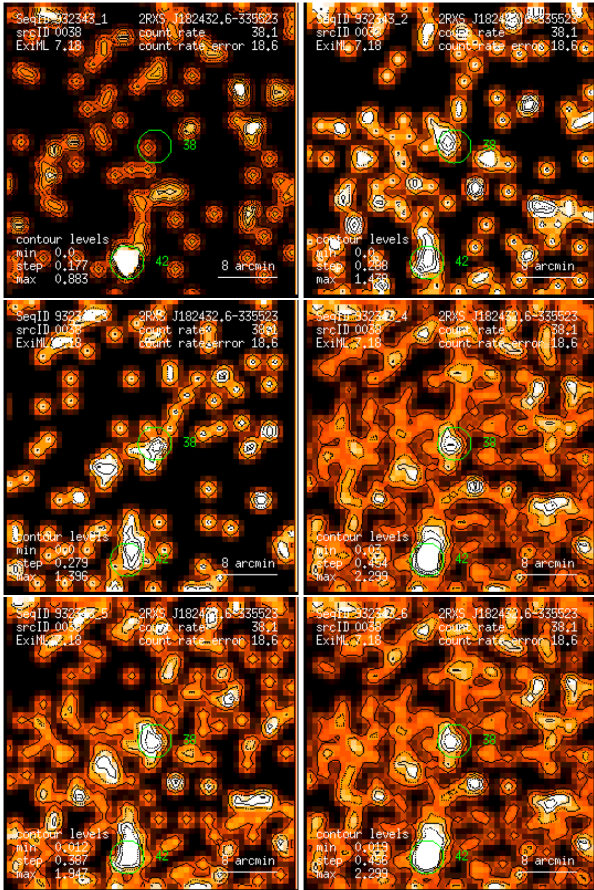
Figure 38: RASS 932343: detection 0038: band rate images, Gaussian filter: (1) PSPC channels 11 – 41, (2) 52 – 90, (3) 91 – 201, (4) 11 – 235, (5) 52 – 201, (6) 11 – 201. Broad band rates in counts/ks. Band rate contour levels in counts/ks/arcmin 2 .
