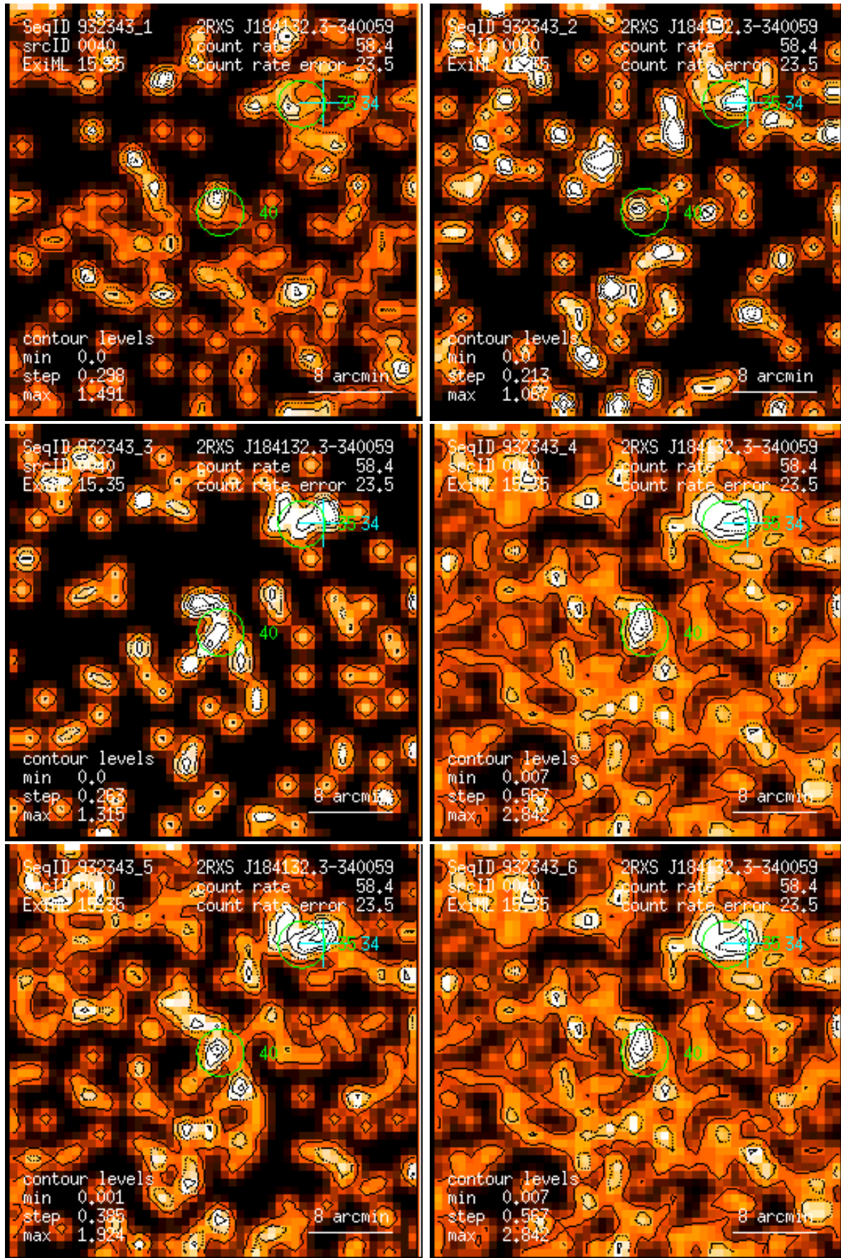
Figure 40: RASS 932343: detection 0040: band rate images, Gaussian filter: (1) PSPC channels 11 – 41, (2) 52 – 90, (3) 91 – 201, (4) 11 – 235, (5) 52 – 201, (6) 11 – 201. Broad band rates in counts/ks. Band rate contour levels in counts/ks/arcmin 2 .
