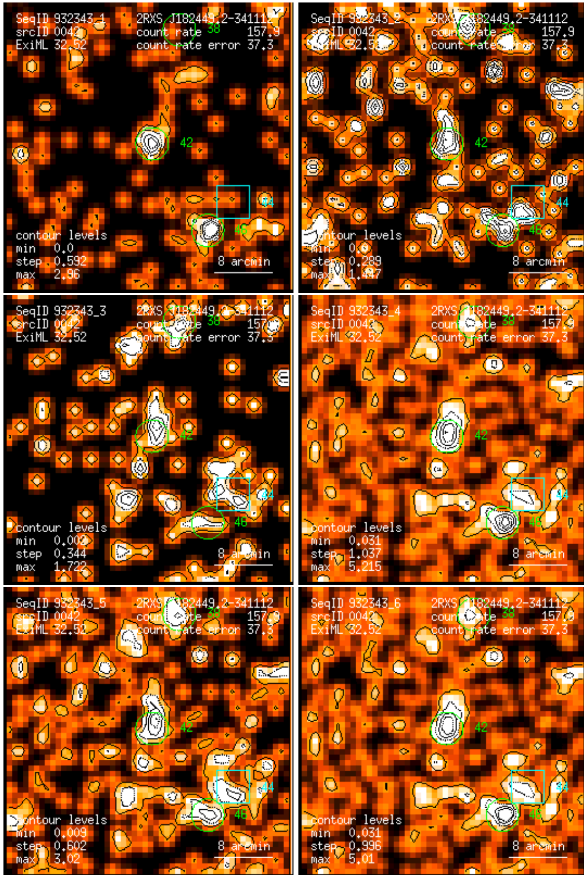
Figure 42: RASS 932343: detection 0042: band rate images, Gaussian filter: (1) PSPC channels 11 – 41, (2) 52 – 90, (3) 91 – 201, (4) 11 – 235, (5) 52 – 201, (6) 11 – 201. Broad band rates in counts/ks. Band rate contour levels in counts/ks/arcmin 2 .
