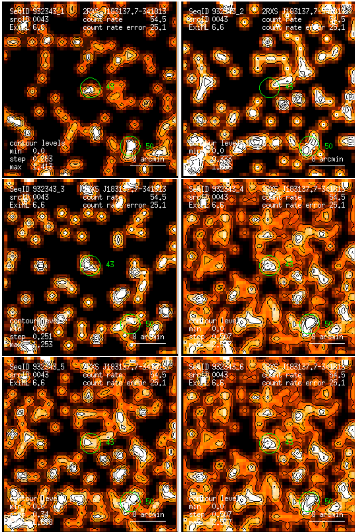
Figure 43: RASS 932343: detection 0043: band rate images, Gaussian filter: (1) PSPC channels 11 – 41, (2) 52 – 90, (3) 91 – 201, (4) 11 – 235, (5) 52 – 201, (6) 11 – 201. Broad band rates in counts/ks. Band rate contour levels in counts/ks/arcmin 2 .
