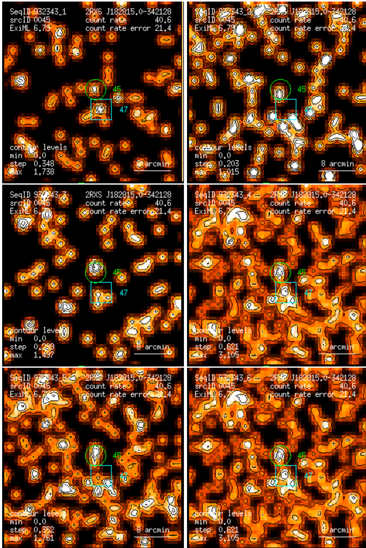
Figure 45: RASS 932343: detection 0045: band rate images, Gaussian filter: (1) PSPC channels 11 – 41, (2) 52 – 90, (3) 91 – 201, (4) 11 – 235, (5) 52 – 201, (6) 11 – 201. Broad band rates in counts/ks. Band rate contour levels in counts/ks/arcmin 2 .
