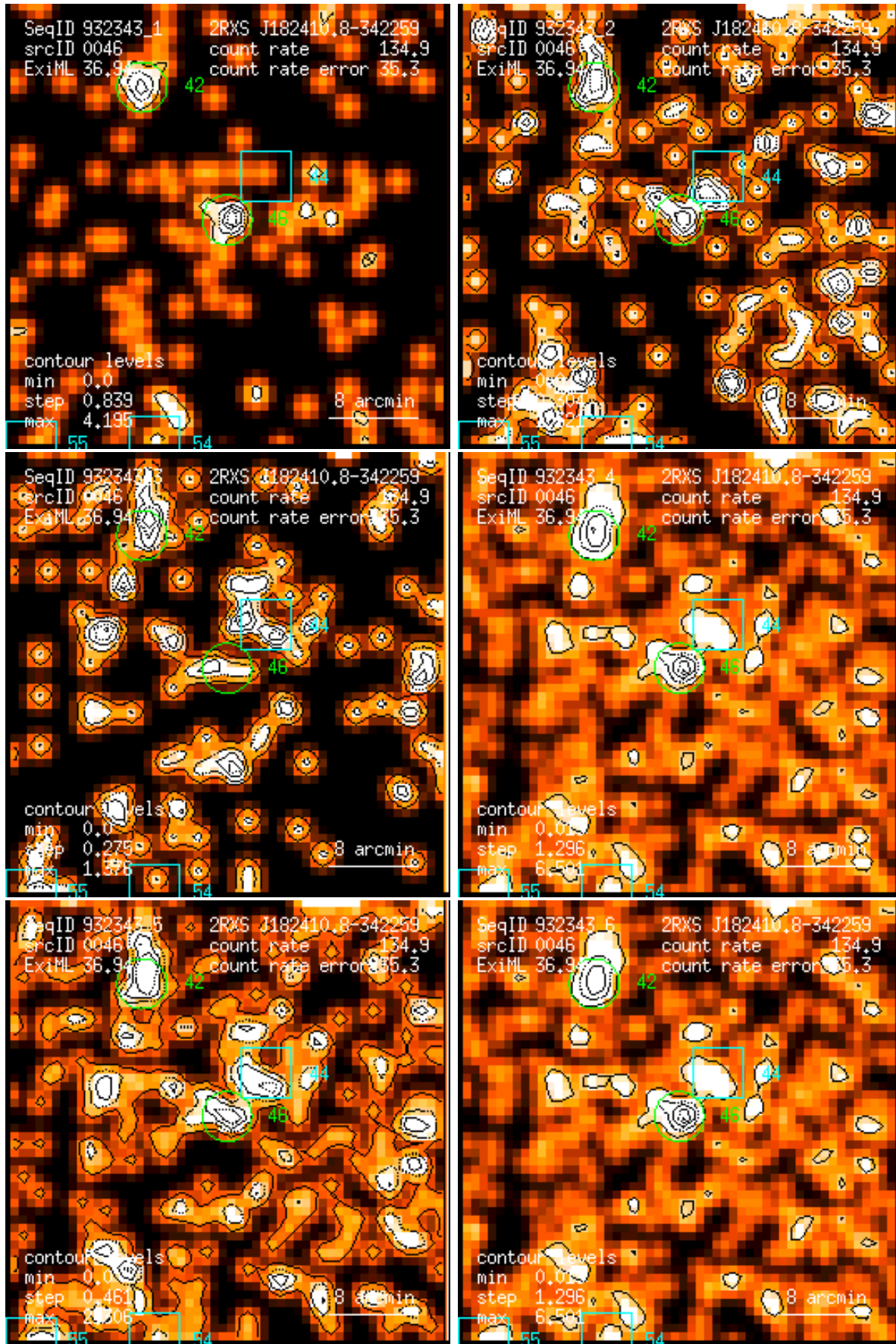
Figure 46: RASS 932343: detection 0046: band rate images, Gaussian filter: (1) PSPC channels 11 – 41, (2) 52 – 90, (3) 91 – 201, (4) 11 – 235, (5) 52 – 201, (6) 11 – 201. Broad band rates in counts/ks. Band rate contour levels in counts/ks/arcmin 2 .
