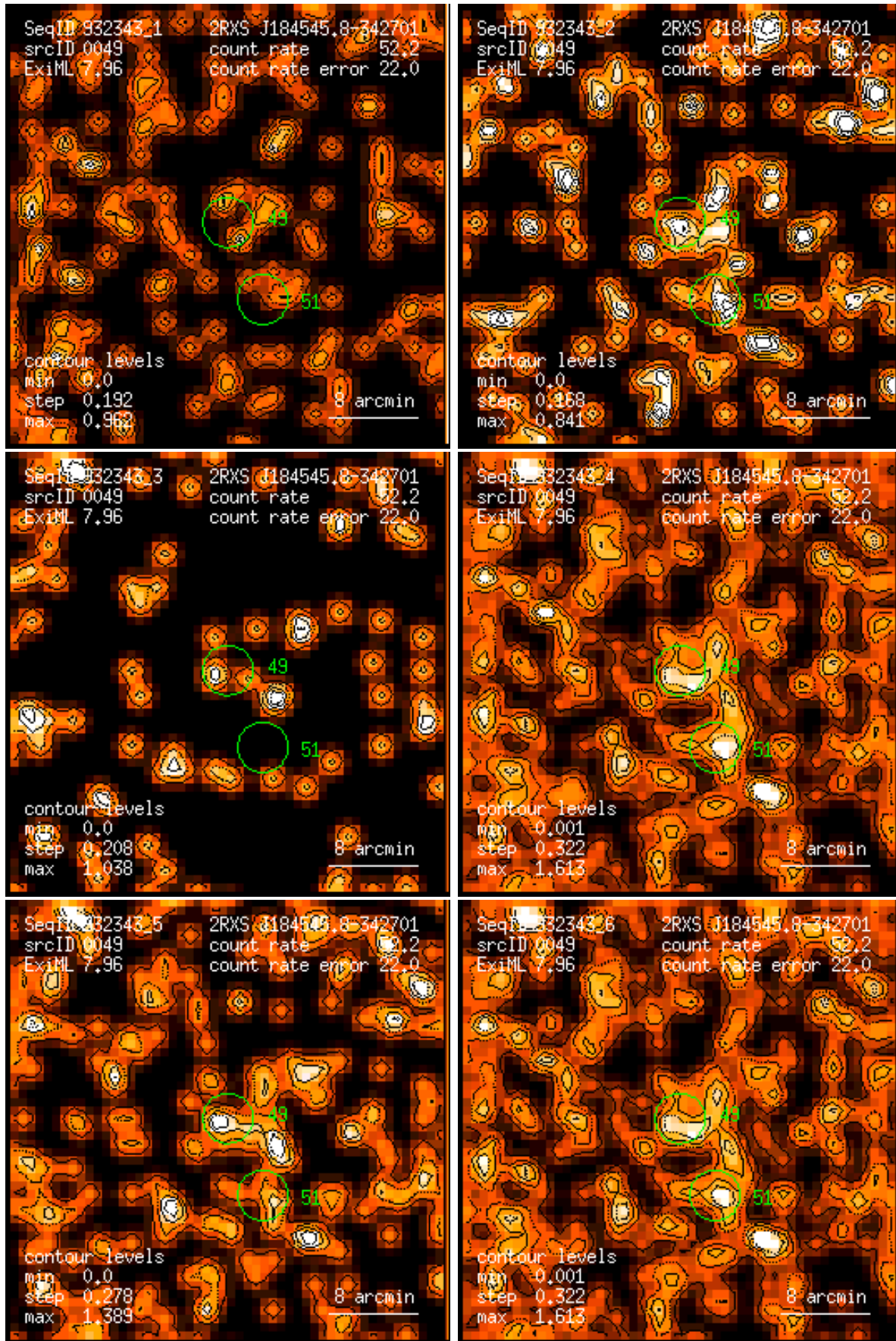
Figure 49: RASS 932343: detection 0049: band rate images, Gaussian filter: (1) PSPC channels 11 – 41, (2) 52 – 90, (3) 91 – 201, (4) 11 – 235, (5) 52 – 201, (6) 11 – 201. Broad band rates in counts/ks. Band rate contour levels in counts/ks/arcmin 2 .
