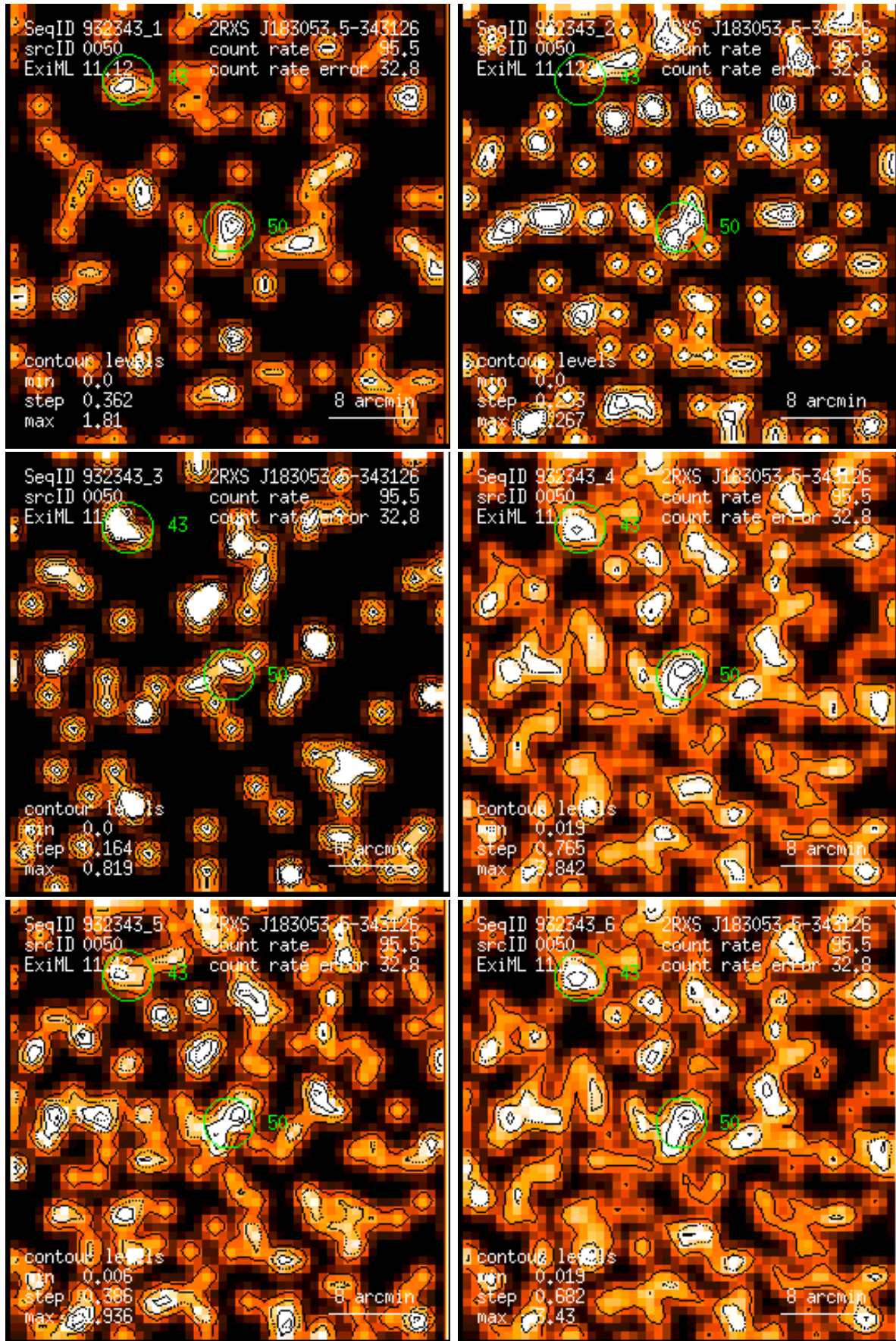
Figure 50: RASS 932343: detection 0050: band rate images, Gaussian filter: (1) PSPC channels 11 – 41, (2) 52 – 90, (3) 91 – 201, (4) 11 – 235, (5) 52 – 201, (6) 11 – 201. Broad band rates in counts/ks. Band rate contour levels in counts/ks/arcmin 2 .
