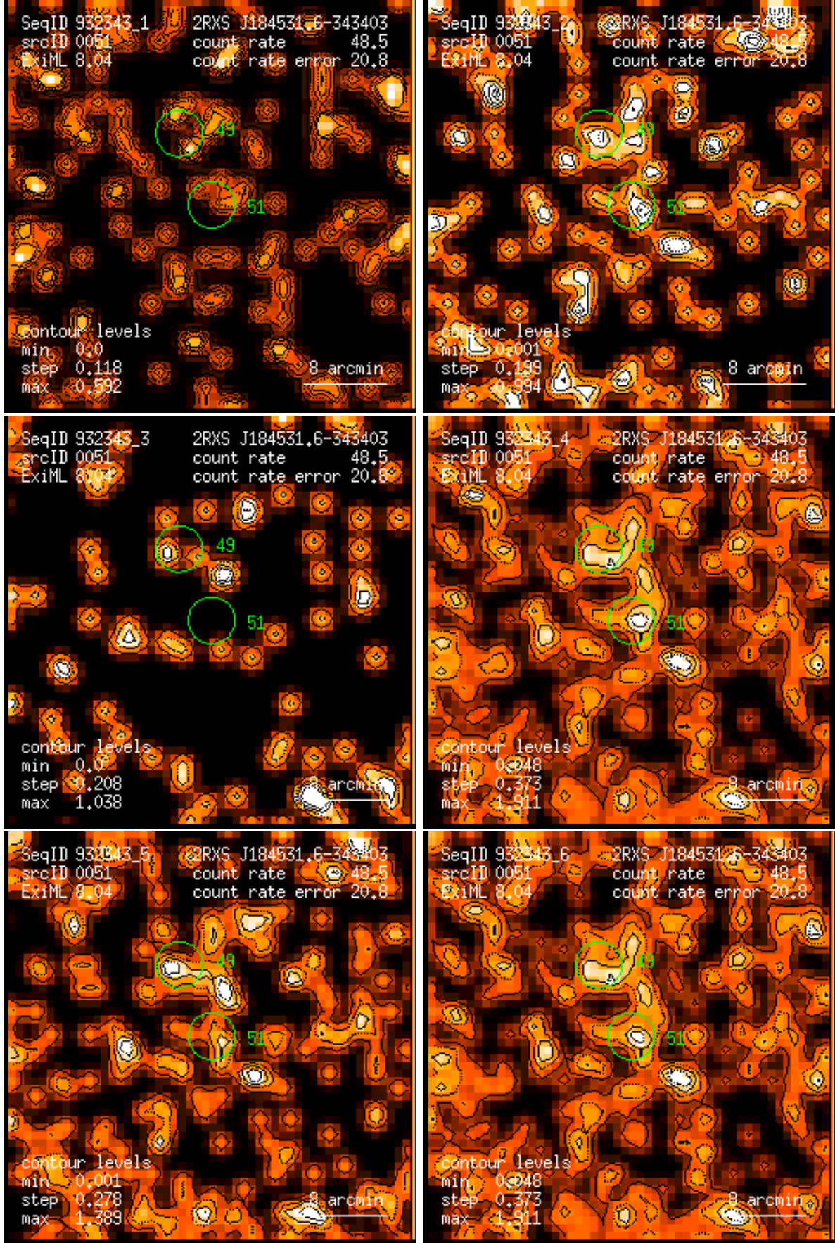
Figure 51: RASS 932343: detection 0051: band rate images, Gaussian filter: (1) PSPC channels 11 – 41, (2) 52 – 90, (3) 91 – 201, (4) 11 – 235, (5) 52 – 201, (6) 11 – 201. Broad band rates in counts/ks. Band rate contour levels in counts/ks/arcmin 2 .
