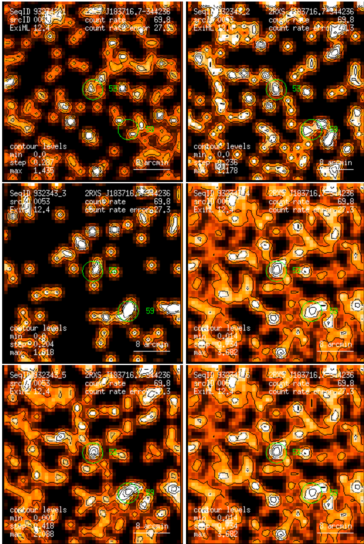
Figure 53: RASS 932343: detection 0053: band rate images, Gaussian filter: (1) PSPC channels 11 – 41, (2) 52 – 90, (3) 91 – 201, (4) 11 – 235, (5) 52 – 201, (6) 11 – 201. Broad band rates in counts/ks. Band rate contour levels in counts/ks/arcmin 2 .
