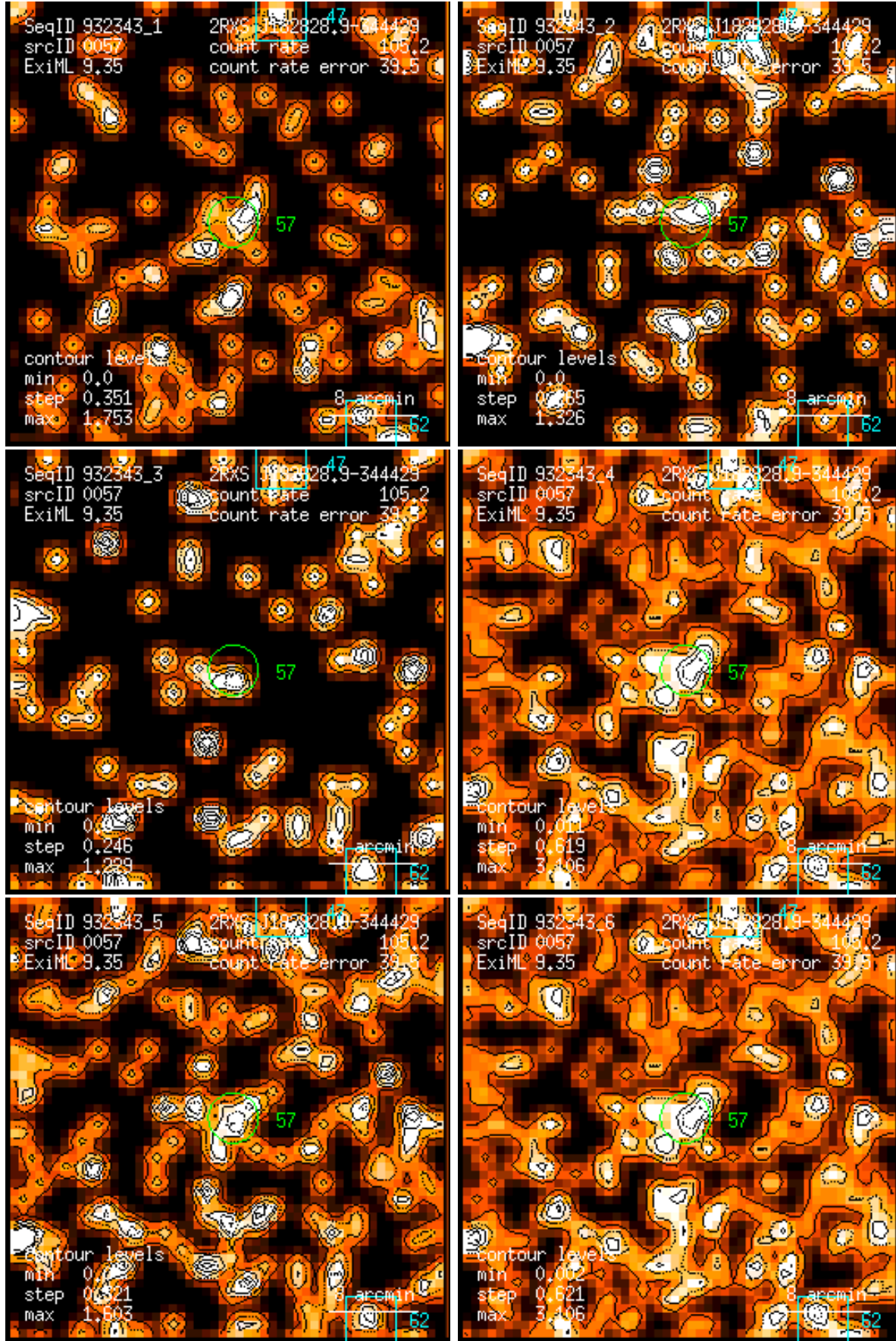
Figure 57: RASS 932343: detection 0057: band rate images, Gaussian filter: (1) PSPC channels 11 – 41, (2) 52 – 90, (3) 91 – 201, (4) 11 – 235, (5) 52 – 201, (6) 11 – 201. Broad band rates in counts/ks. Band rate contour levels in counts/ks/arcmin 2 .
