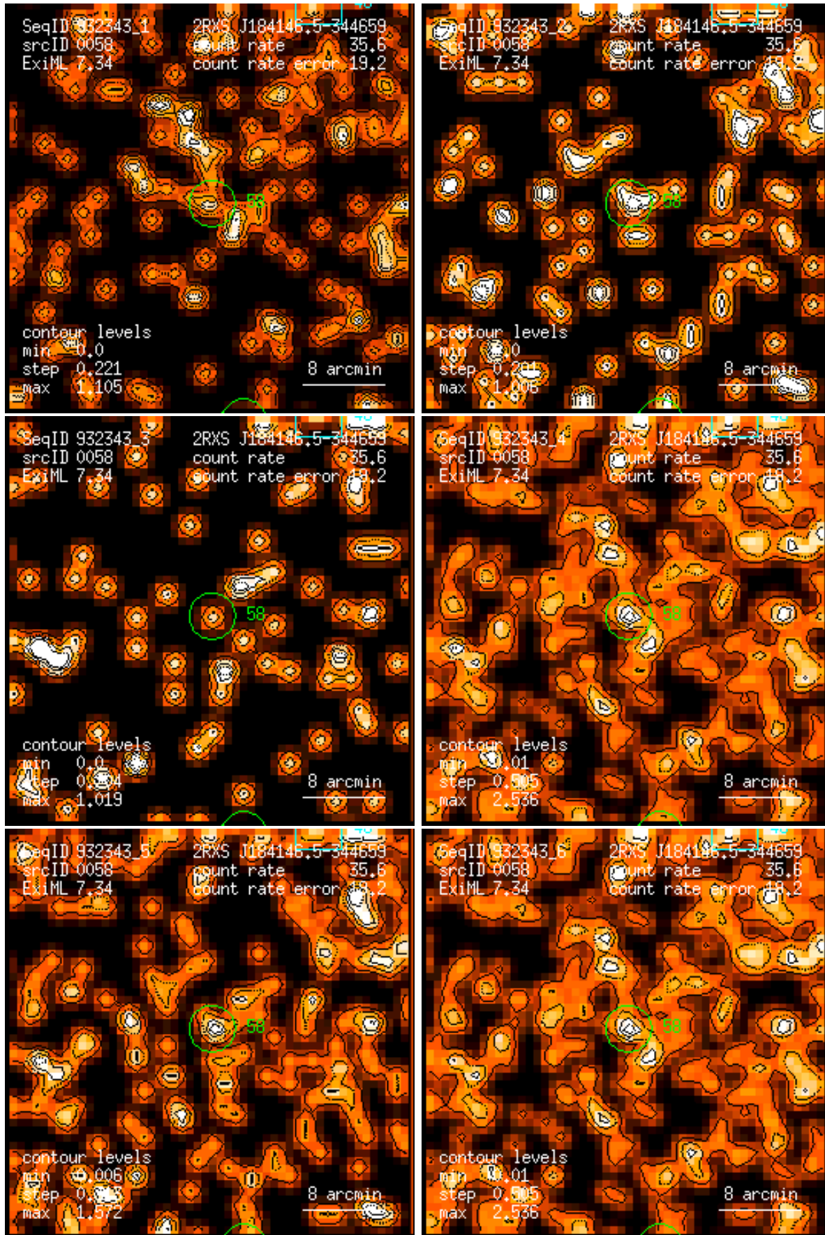
Figure 58: RASS 932343: detection 0058: band rate images, Gaussian filter: (1) PSPC channels 11 – 41, (2) 52 – 90, (3) 91 – 201, (4) 11 – 235, (5) 52 – 201, (6) 11 – 201. Broad band rates in counts/ks. Band rate contour levels in counts/ks/arcmin 2 .
