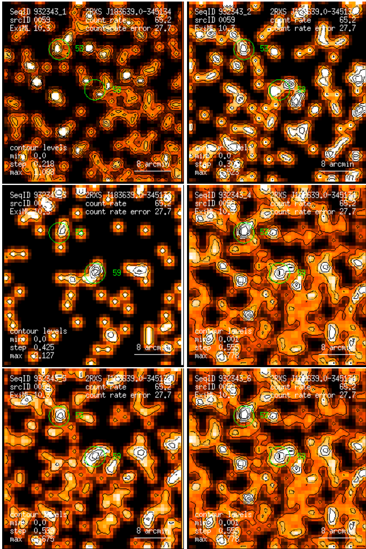
Figure 59: RASS 932343: detection 0059: band rate images, Gaussian filter: (1) PSPC channels 11 – 41, (2) 52 – 90, (3) 91 – 201, (4) 11 – 235, (5) 52 – 201, (6) 11 – 201. Broad band rates in counts/ks. Band rate contour levels in counts/ks/arcmin 2 .
