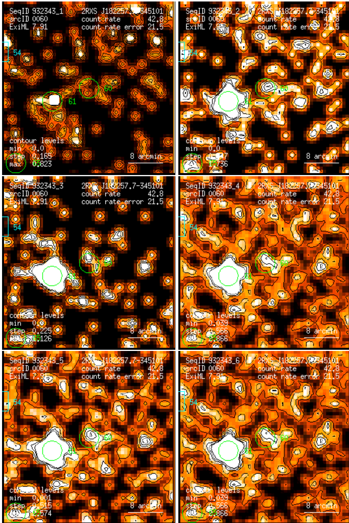
Figure 60: RASS 932343: detection 0060: band rate images, Gaussian filter: (1) PSPC channels 11 – 41, (2) 52 – 90, (3) 91 – 201, (4) 11 – 235, (5) 52 – 201, (6) 11 – 201. Broad band rates in counts/ks. Band rate contour levels in counts/ks/arcmin 2 .
