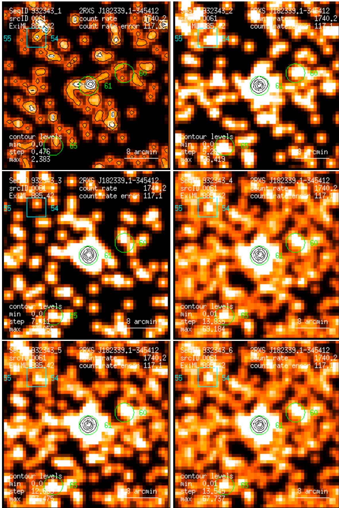
Figure 61: RASS 932343: detection 0061: band rate images, Gaussian filter: (1) PSPC channels 11 – 41, (2) 52 – 90, (3) 91 – 201, (4) 11 – 235, (5) 52 – 201, (6) 11 – 201. Broad band rates in counts/ks. Band rate contour levels in counts/ks/arcmin 2 .
