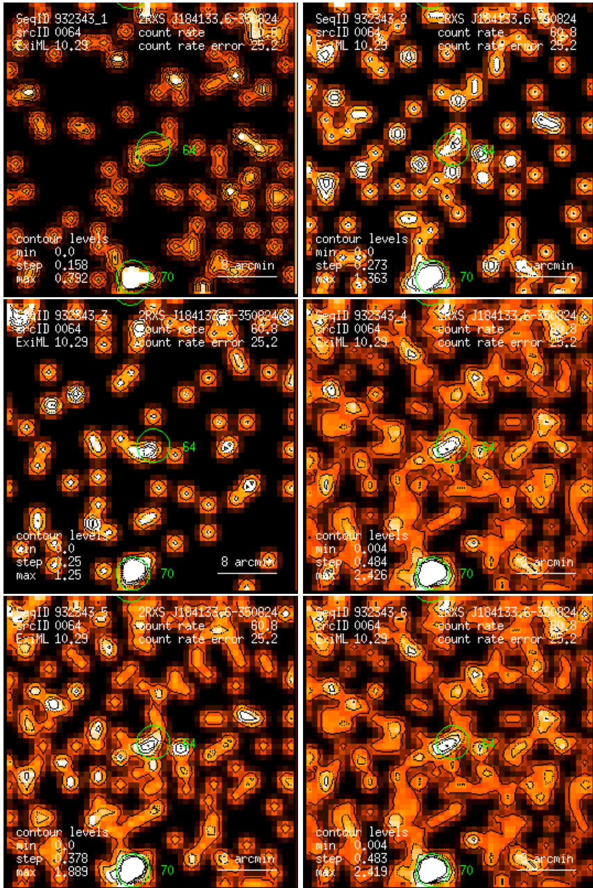
Figure 64: RASS 932343: detection 0064: band rate images, Gaussian filter: (1) PSPC channels 11 – 41, (2) 52 – 90, (3) 91 – 201, (4) 11 – 235, (5) 52 – 201, (6) 11 – 201. Broad band rates in counts/ks. Band rate contour levels in counts/ks/arcmin 2 .
