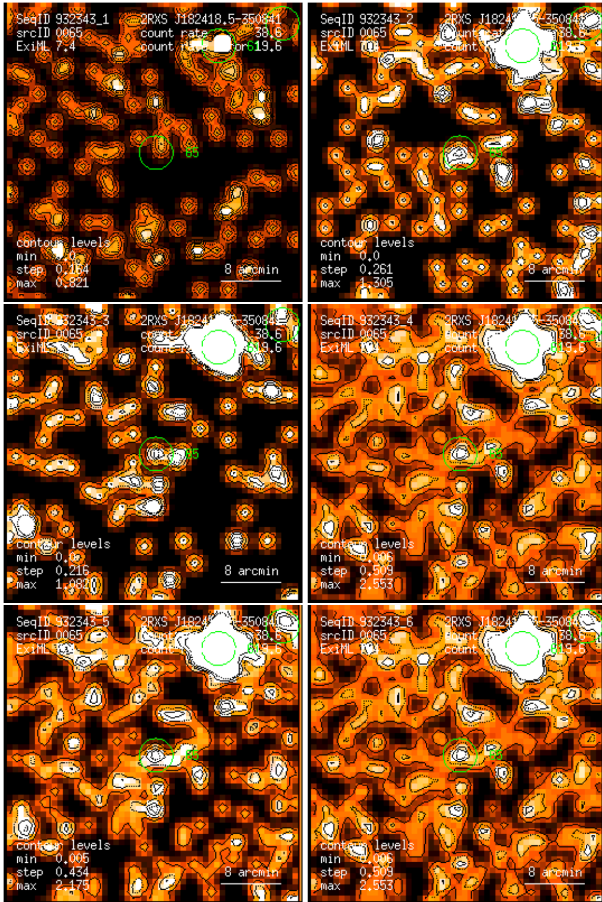
Figure 65: RASS 932343: detection 0065: band rate images, Gaussian filter: (1) PSPC channels 11 – 41, (2) 52 – 90, (3) 91 – 201, (4) 11 – 235, (5) 52 – 201, (6) 11 – 201. Broad band rates in counts/ks. Band rate contour levels in counts/ks/arcmin 2 .
