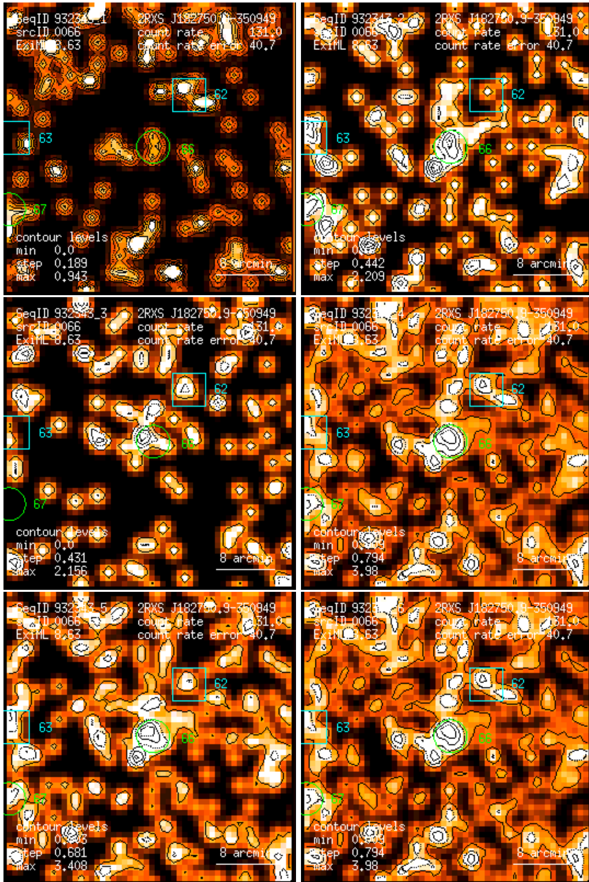
Figure 66: RASS 932343: detection 0066: band rate images, Gaussian filter: (1) PSPC channels 11 – 41, (2) 52 – 90, (3) 91 – 201, (4) 11 – 235, (5) 52 – 201, (6) 11 – 201. Broad band rates in counts/ks. Band rate contour levels in counts/ks/arcmin 2 .
