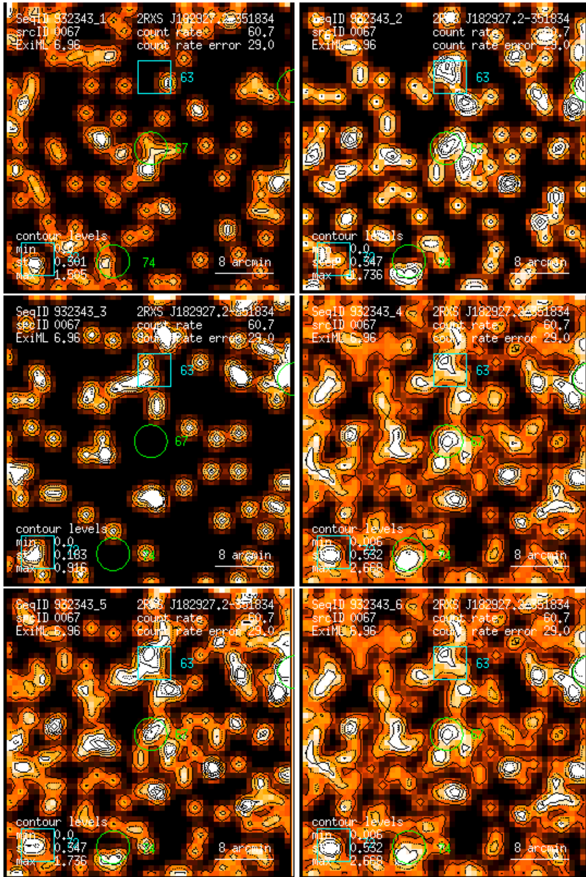
Figure 67: RASS 932343: detection 0067: band rate images, Gaussian filter: (1) PSPC channels 11 – 41, (2) 52 – 90, (3) 91 – 201, (4) 11 – 235, (5) 52 – 201, (6) 11 – 201. Broad band rates in counts/ks. Band rate contour levels in counts/ks/arcmin 2 .
