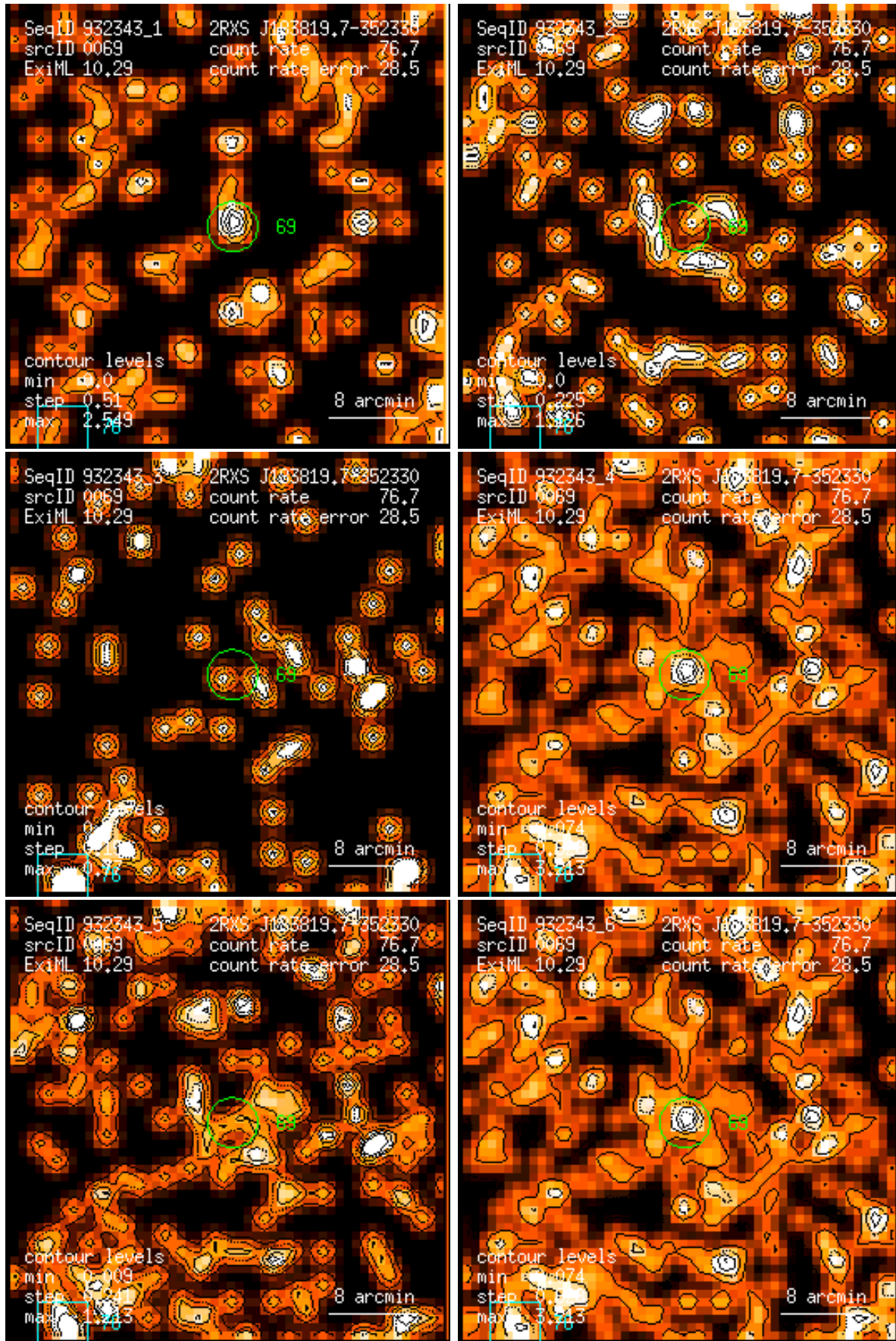
Figure 69: RASS 932343: detection 0069: band rate images, Gaussian filter: (1) PSPC channels 11 – 41, (2) 52 – 90, (3) 91 – 201, (4) 11 – 235, (5) 52 – 201, (6) 11 – 201. Broad band rates in counts/ks. Band rate contour levels in counts/ks/arcmin 2 .
