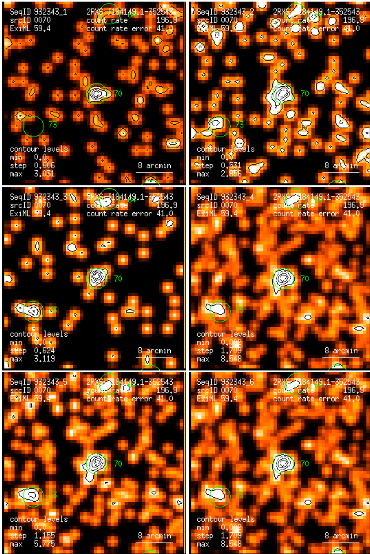
Figure 70: RASS 932343: detection 0070: band rate images, Gaussian filter: (1) PSPC channels 11 – 41, (2) 52 – 90, (3) 91 – 201, (4) 11 – 235, (5) 52 – 201, (6) 11 – 201. Broad band rates in counts/ks. Band rate contour levels in counts/ks/arcmin 2 .
