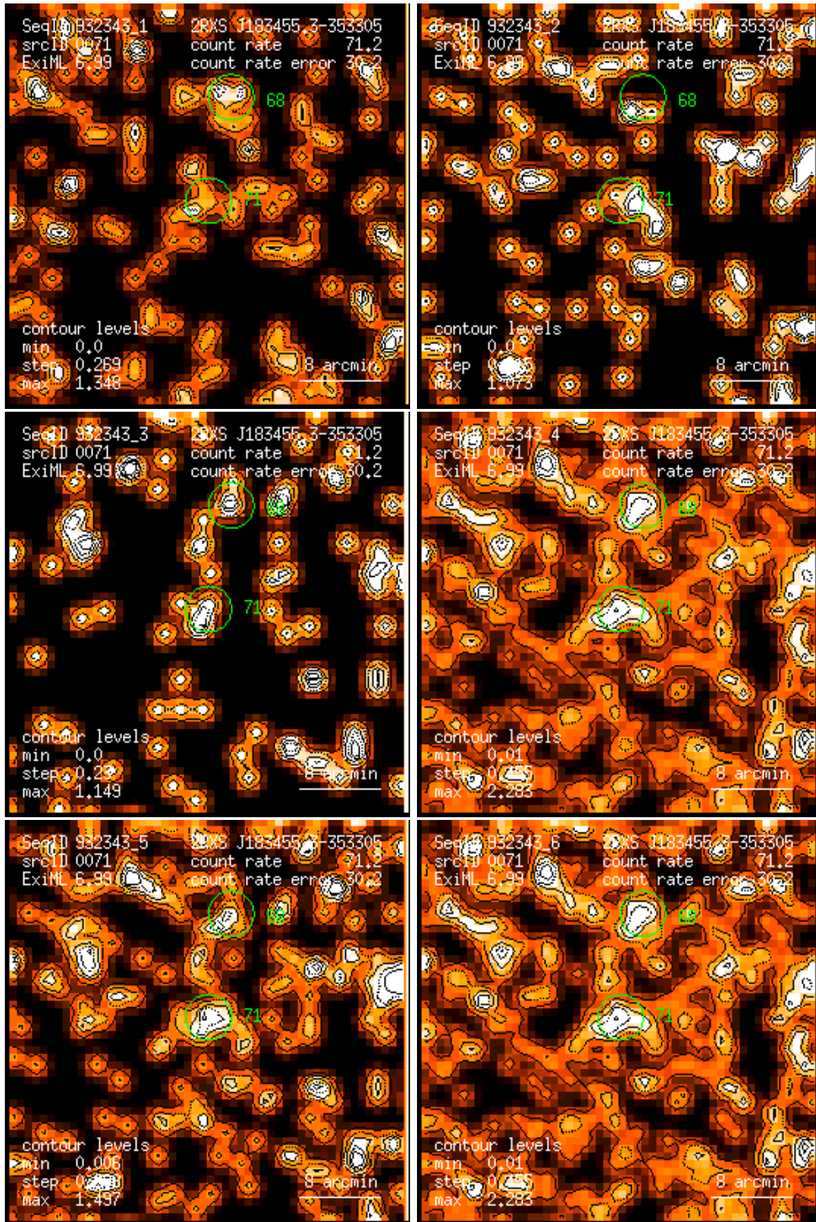
Figure 71: RASS 932343: detection 0071: band rate images, Gaussian filter: (1) PSPC channels 11 – 41, (2) 52 – 90, (3) 91 – 201, (4) 11 – 235, (5) 52 – 201, (6) 11 – 201. Broad band rates in counts/ks. Band rate contour levels in counts/ks/arcmin 2 .
