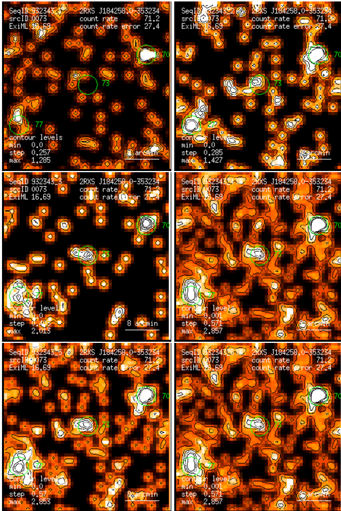
Figure 73: RASS 932343: detection 0073: band rate images, Gaussian filter: (1) PSPC channels 11 – 41, (2) 52 – 90, (3) 91 – 201, (4) 11 – 235, (5) 52 – 201, (6) 11 – 201. Broad band rates in counts/ks. Band rate contour levels in counts/ks/arcmin 2 .
