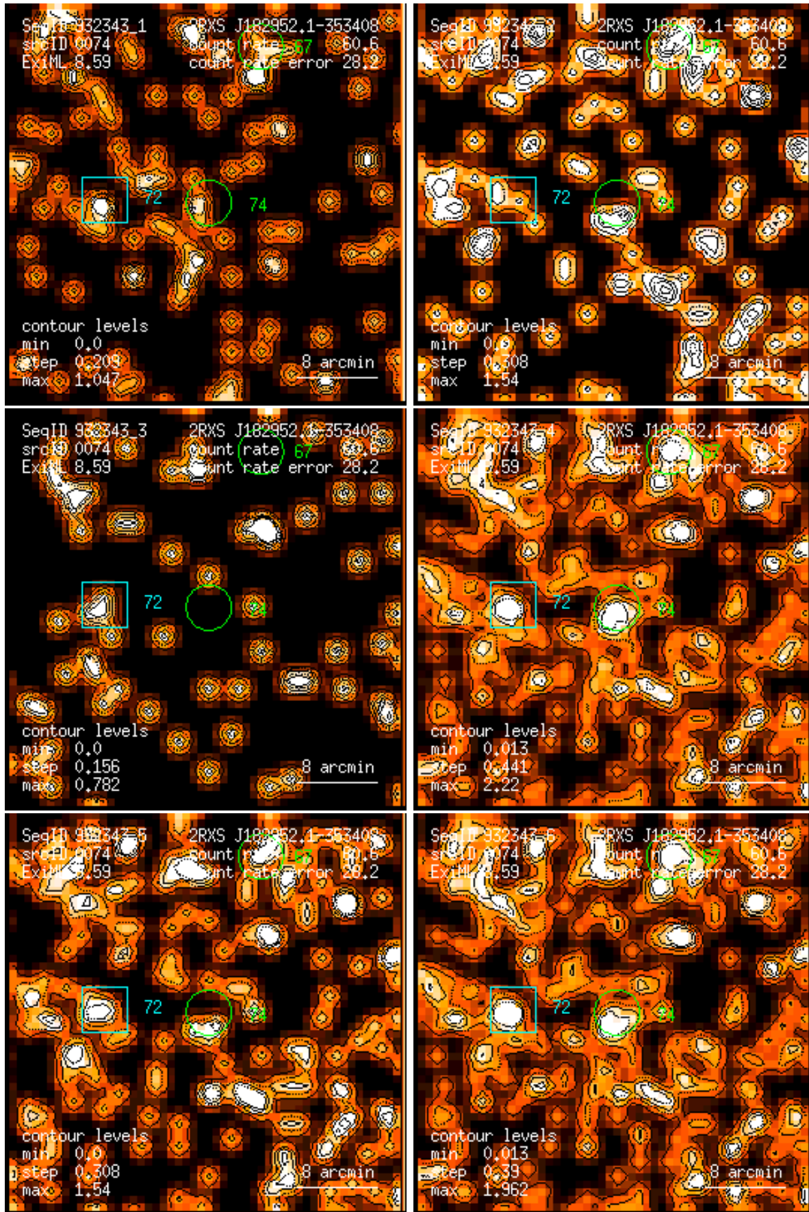
Figure 74: RASS 932343: detection 0074: band rate images, Gaussian filter: (1) PSPC channels 11 – 41, (2) 52 – 90, (3) 91 – 201, (4) 11 – 235, (5) 52 – 201, (6) 11 – 201. Broad band rates in counts/ks. Band rate contour levels in counts/ks/arcmin 2 .
