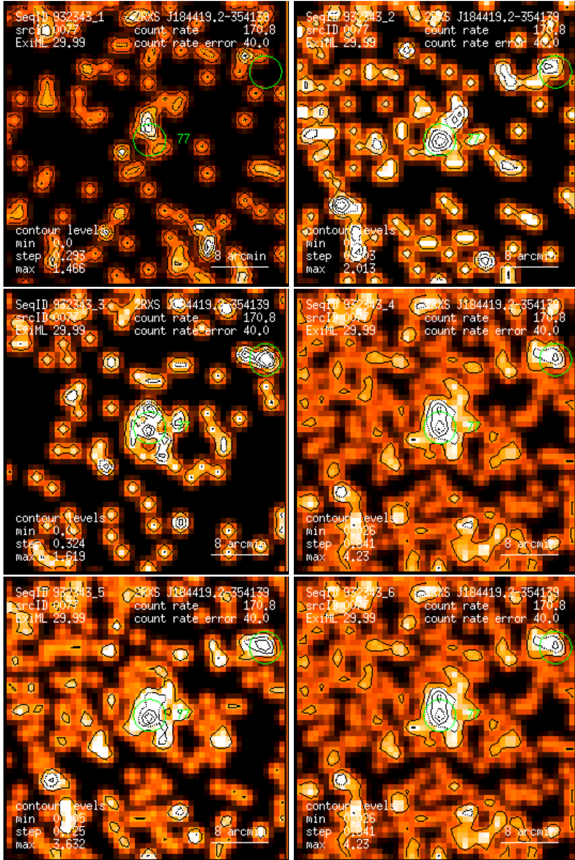
Figure 77: RASS 932343: detection 0077: band rate images, Gaussian filter: (1) PSPC channels 11 – 41, (2) 52 – 90, (3) 91 – 201, (4) 11 – 235, (5) 52 – 201, (6) 11 – 201. Broad band rates in counts/ks. Band rate contour levels in counts/ks/arcmin 2 .
