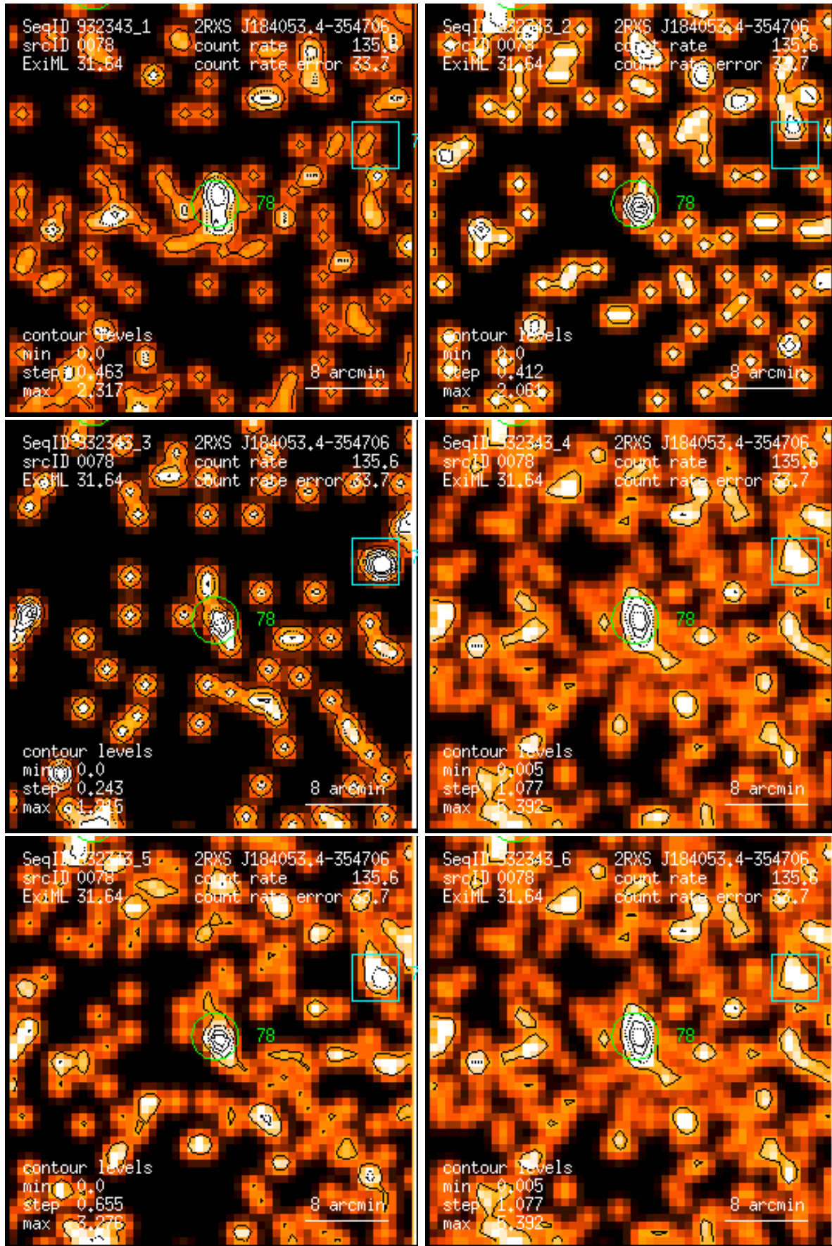
Figure 78: RASS 932343: detection 0078: band rate images, Gaussian filter: (1) PSPC channels 11 – 41, (2) 52 – 90, (3) 91 – 201, (4) 11 – 235, (5) 52 – 201, (6) 11 – 201. Broad band rates in counts/ks. Band rate contour levels in counts/ks/arcmin 2 .
