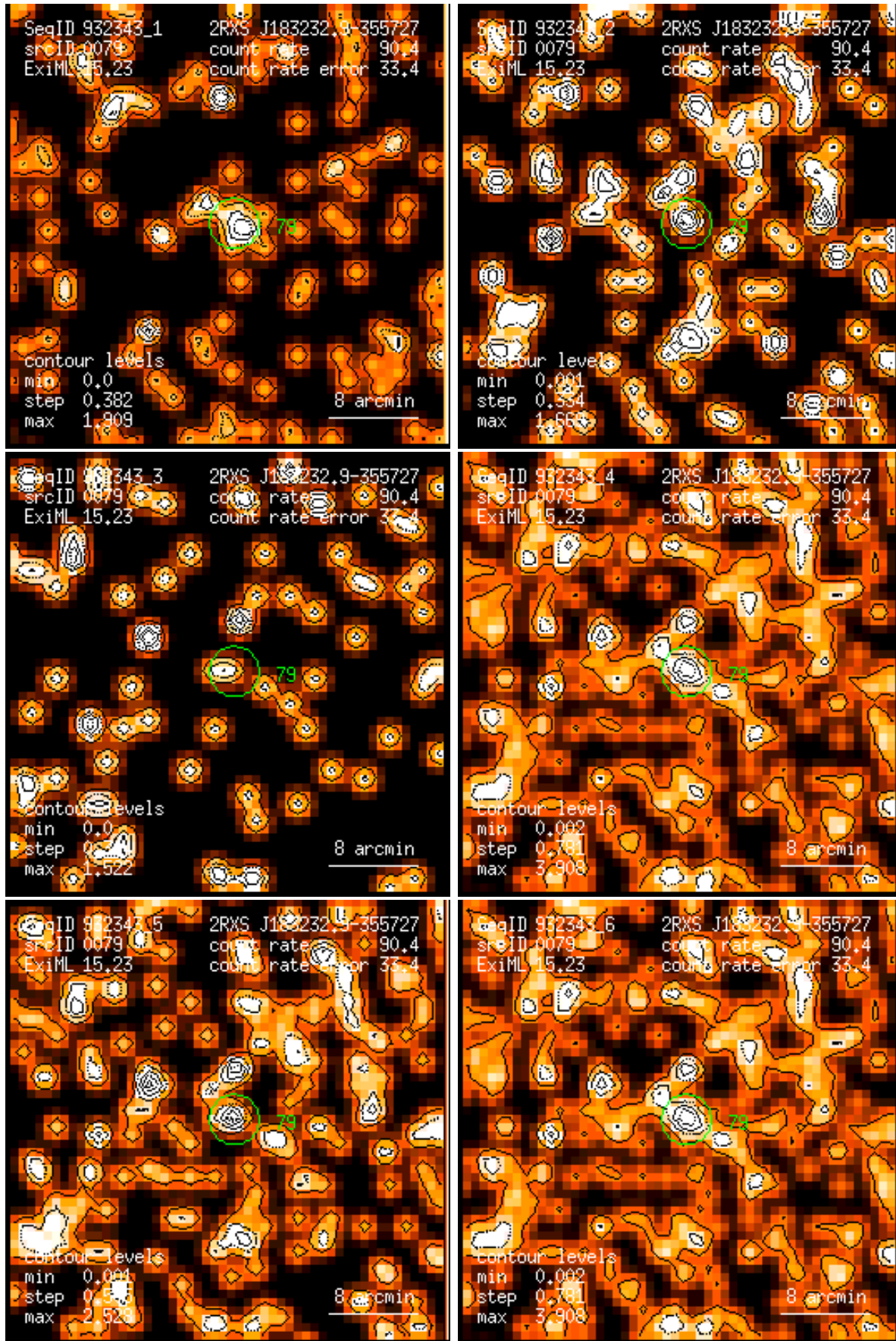
Figure 79: RASS 932343: detection 0079: band rate images, Gaussian filter: (1) PSPC channels 11 – 41, (2) 52 – 90, (3) 91 – 201, (4) 11 – 235, (5) 52 – 201, (6) 11 – 201. Broad band rates in counts/ks. Band rate contour levels in counts/ks/arcmin 2 .
