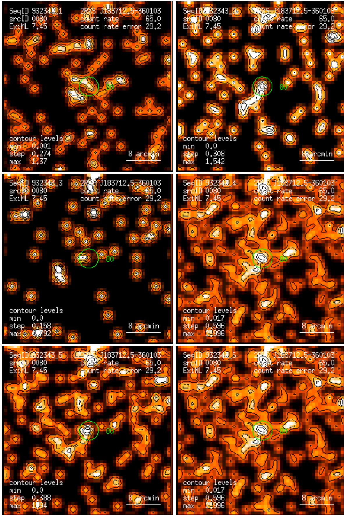
Figure 80: RASS 932343: detection 0080: band rate images, Gaussian filter: (1) PSPC channels 11 – 41, (2) 52 – 90, (3) 91 – 201, (4) 11 – 235, (5) 52 – 201, (6) 11 – 201. Broad band rates in counts/ks. Band rate contour levels in counts/ks/arcmin 2 .
