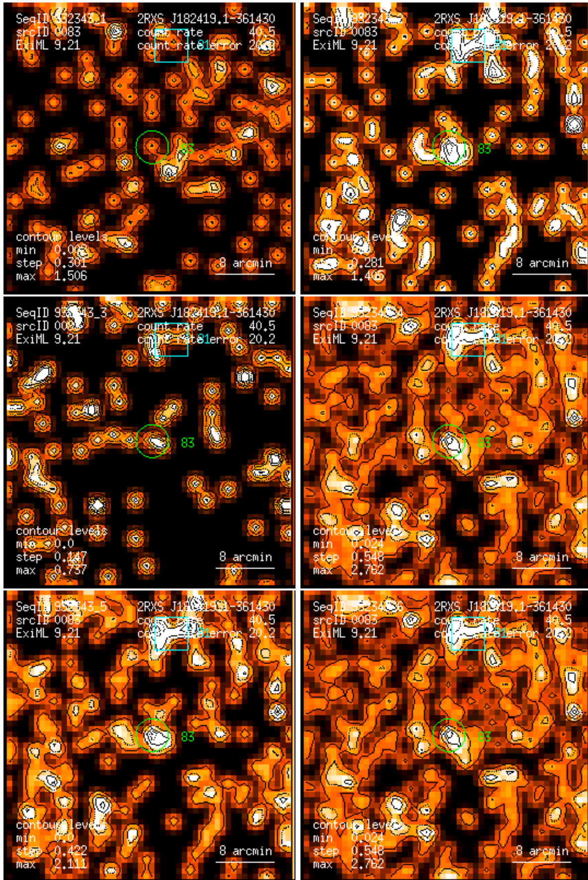
Figure 83: RASS 932343: detection 0083: band rate images, Gaussian filter: (1) PSPC channels 11 – 41, (2) 52 – 90, (3) 91 – 201, (4) 11 – 235, (5) 52 – 201, (6) 11 – 201. Broad band rates in counts/ks. Band rate contour levels in counts/ks/arcmin 2 .
