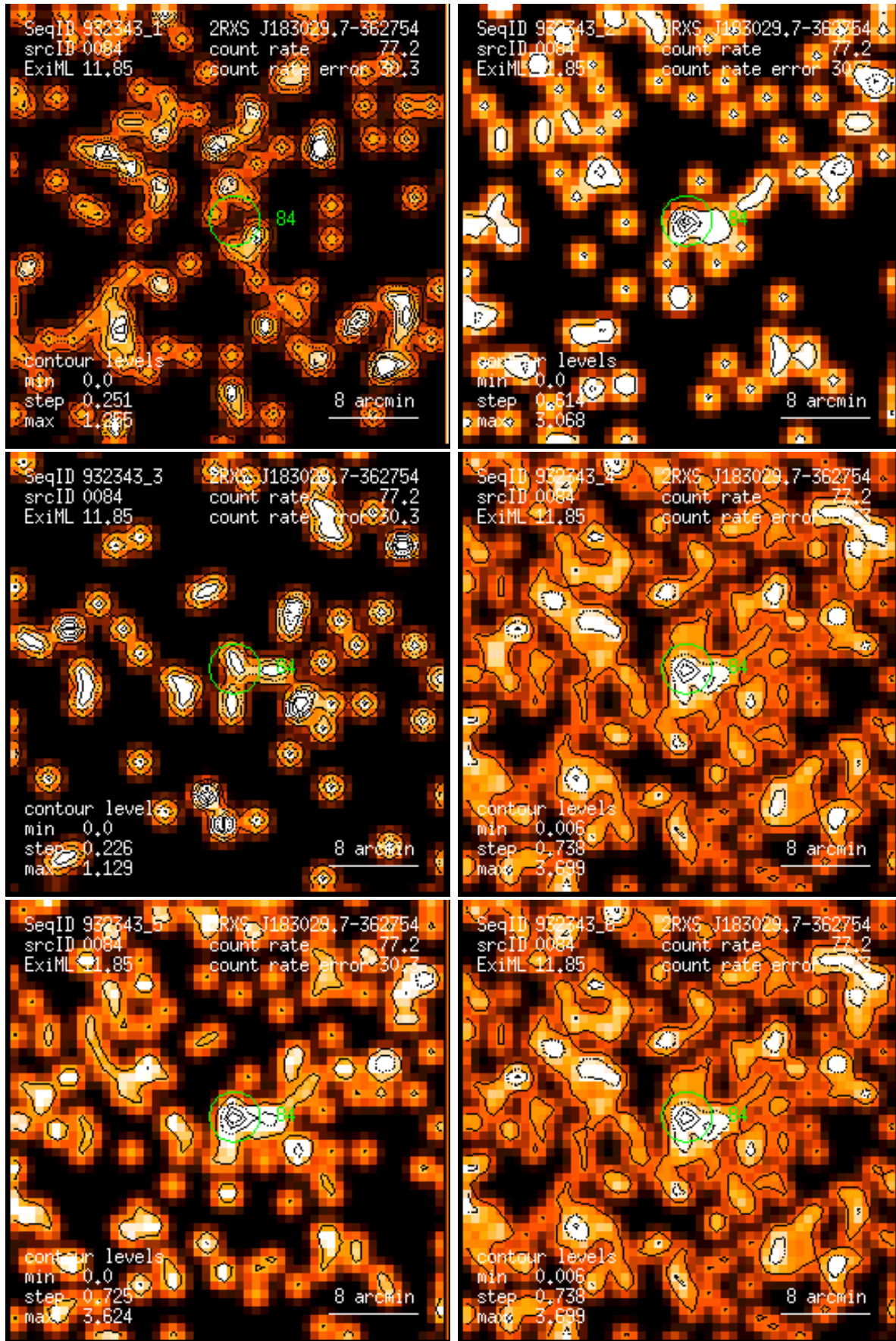
Figure 84: RASS 932343: detection 0084: band rate images, Gaussian filter: (1) PSPC channels 11 – 41, (2) 52 – 90, (3) 91 – 201, (4) 11 – 235, (5) 52 – 201, (6) 11 – 201. Broad band rates in counts/ks. Band rate contour levels in counts/ks/arcmin 2 .
