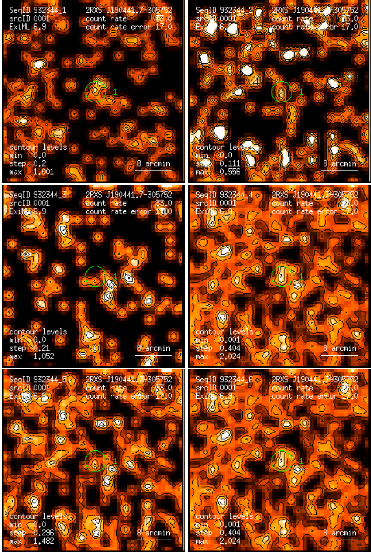
Figure 1: RASS 932344: detection 0001: band rate images, Gaussian filter: (1) PSPC channels 11 – 41, (2) 52 – 90, (3) 91 – 201, (4) 11 – 235, (5) 52 – 201, (6) 11 – 201. Broad band rates in counts/ks. Band rate contour levels in counts/ks/arcmin 2 .
