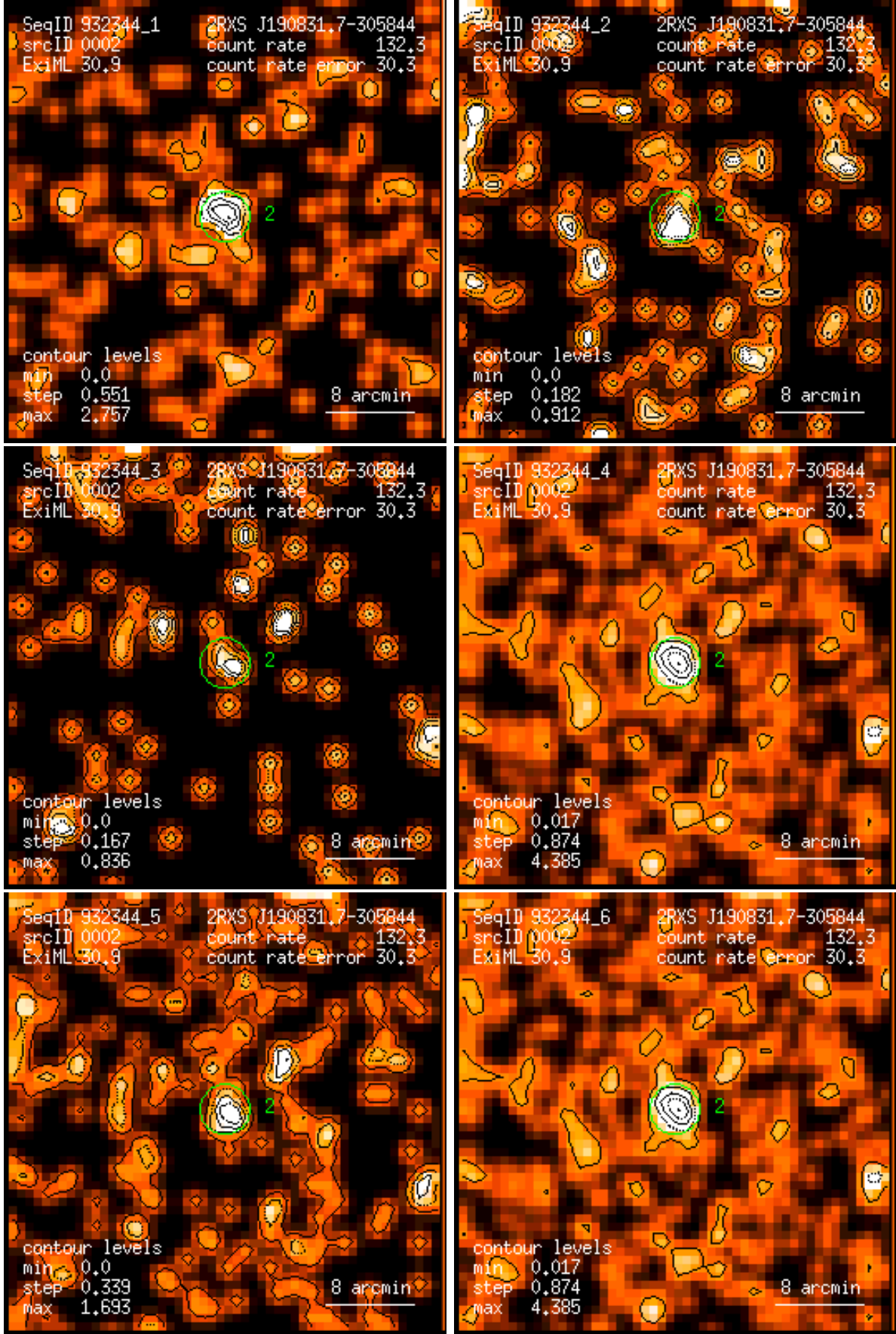
Figure 2: RASS 932344: detection 0002: band rate images, Gaussian filter: (1) PSPC channels 11 – 41, (2) 52 – 90, (3) 91 – 201, (4) 11 – 235, (5) 52 – 201, (6) 11 – 201. Broad band rates in counts/ks. Band rate contour levels in counts/ks/arcmin 2 .
