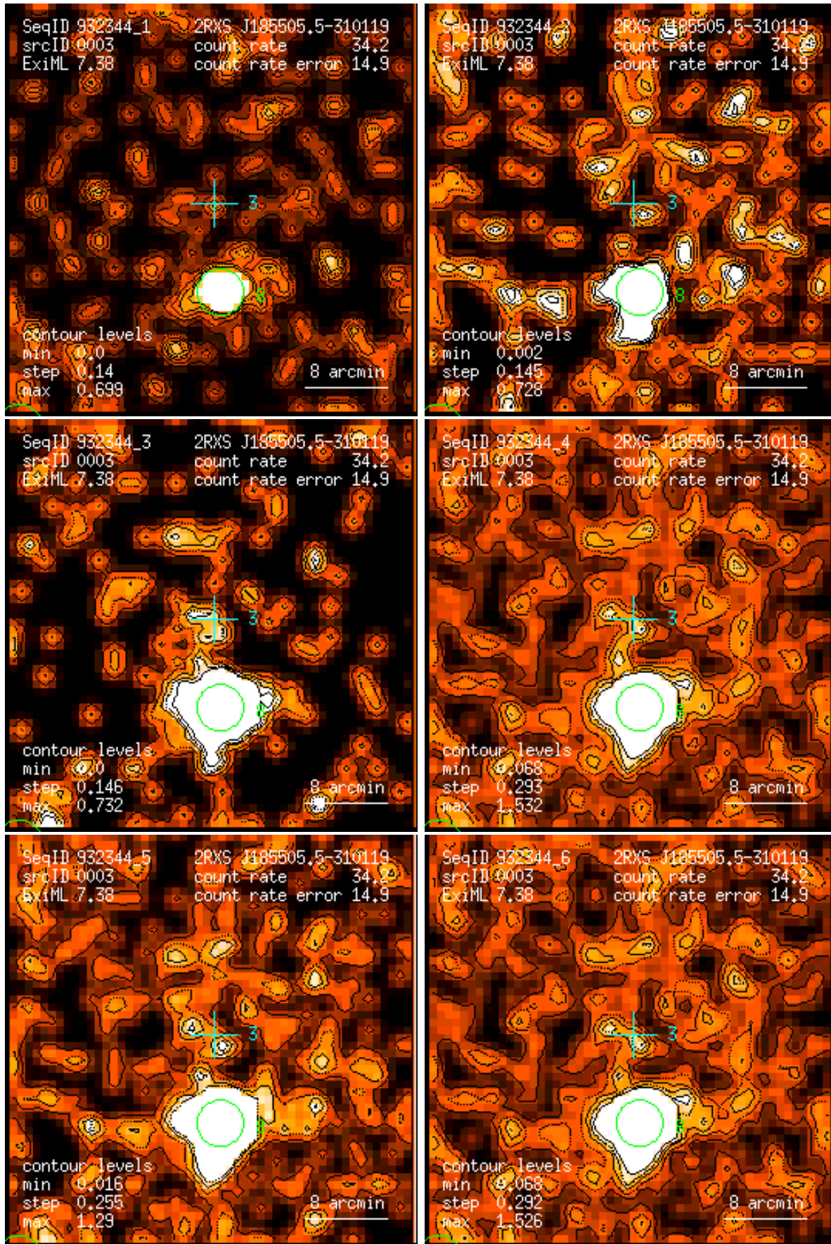
Figure 3: RASS 932344: detection 0003: band rate images, Gaussian filter: (1) PSPC channels 11 – 41, (2) 52 – 90, (3) 91 – 201, (4) 11 – 235, (5) 52 – 201, (6) 11 – 201. Broad band rates in counts/ks. Band rate contour levels in counts/ks/arcmin 2 .
